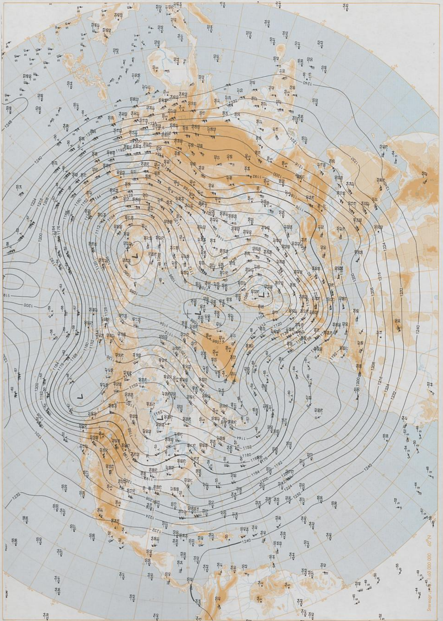
200 hPa 12 UTC
