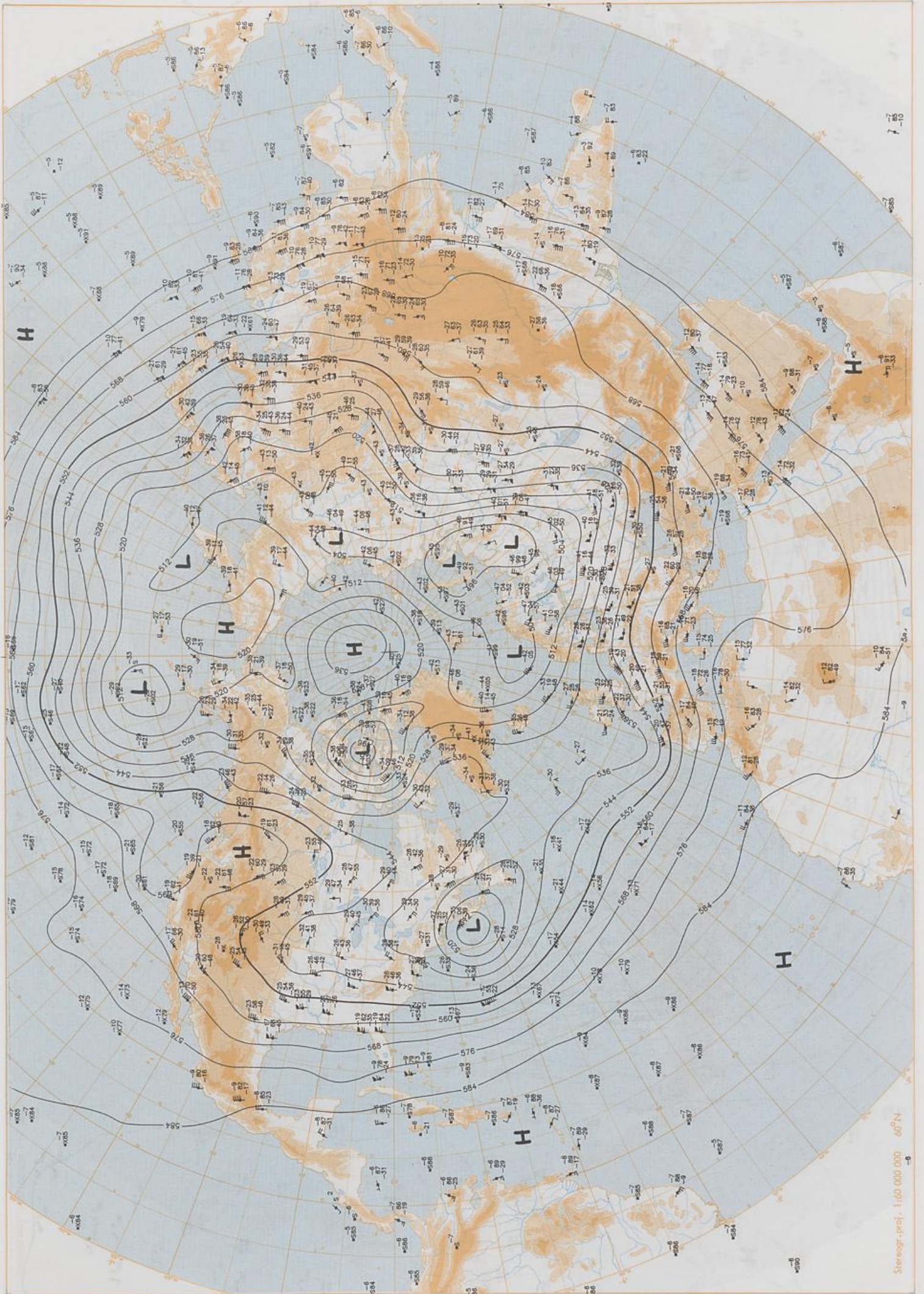
500 hPa 12 UTC
