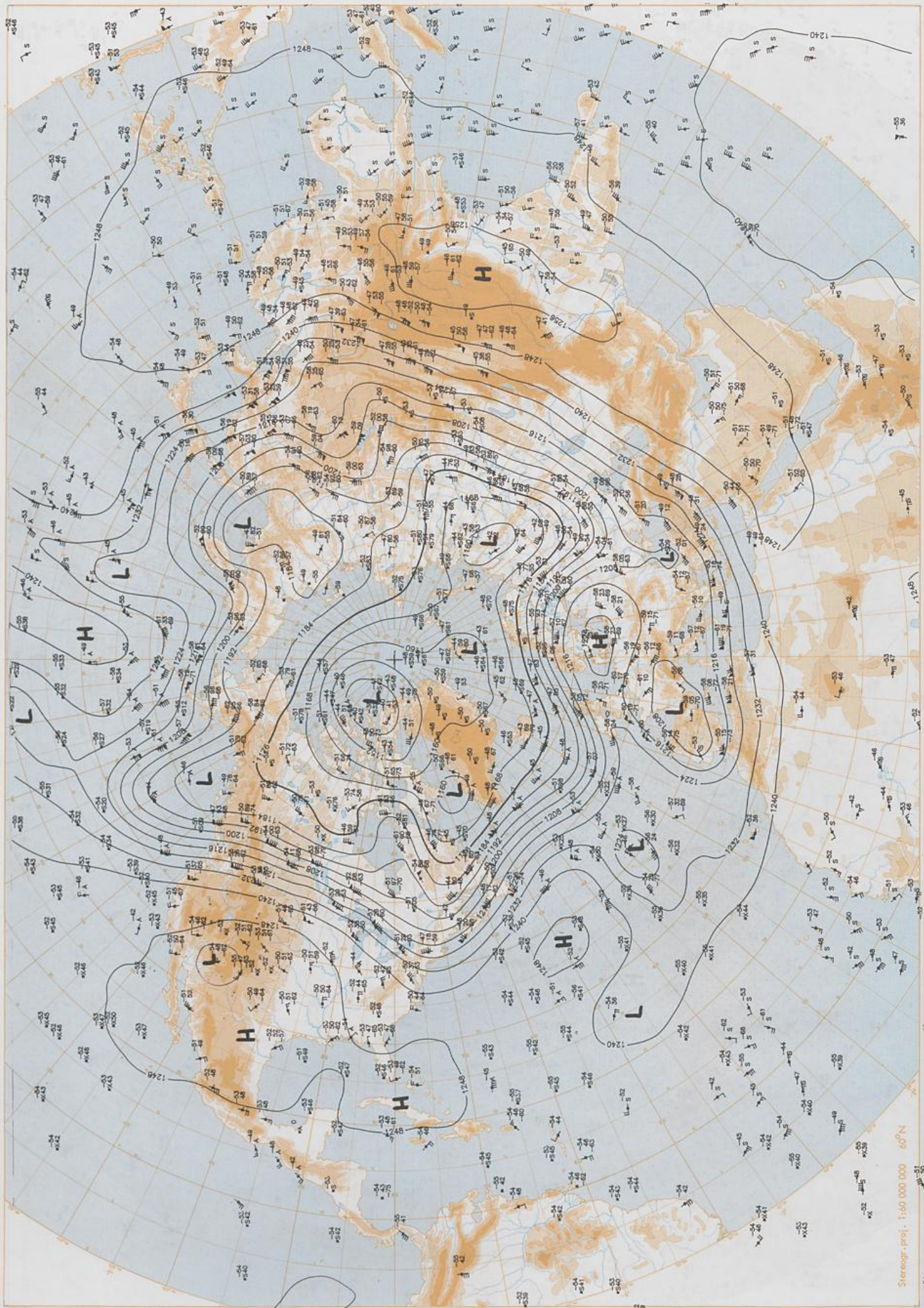
200 hPa 12 UTC
