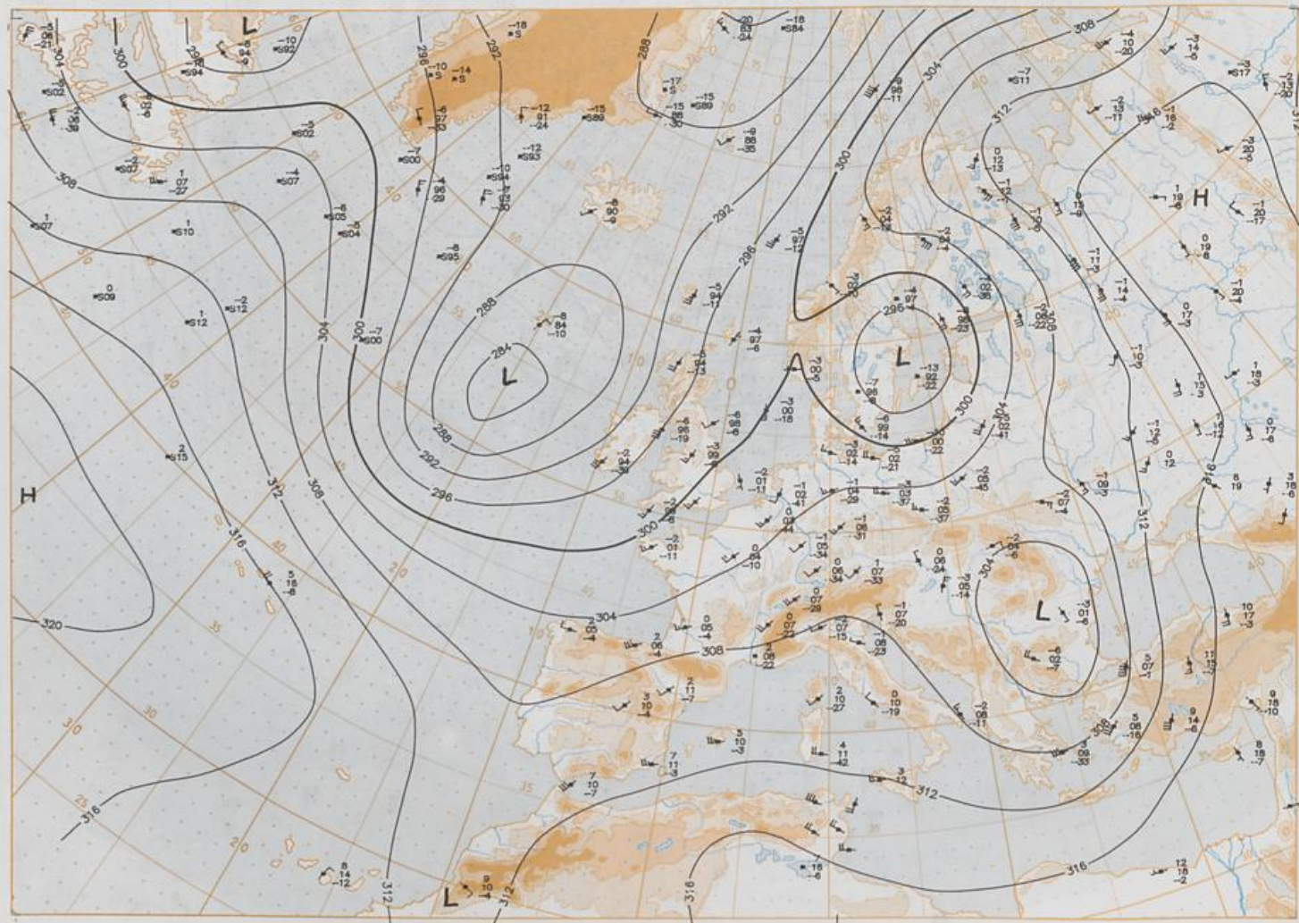
700 hPa 12 UTC
