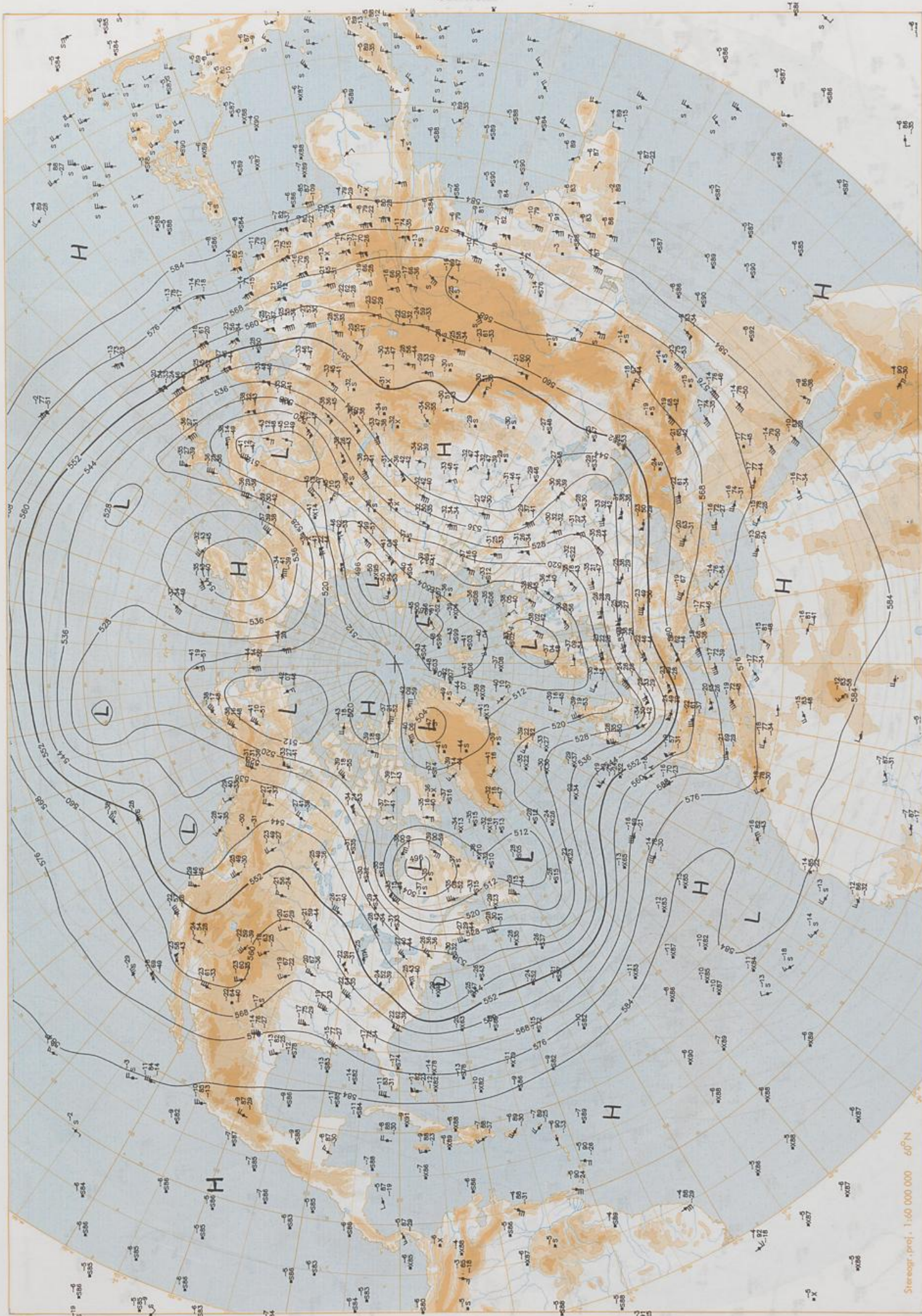
500 hPa 12 UTC
