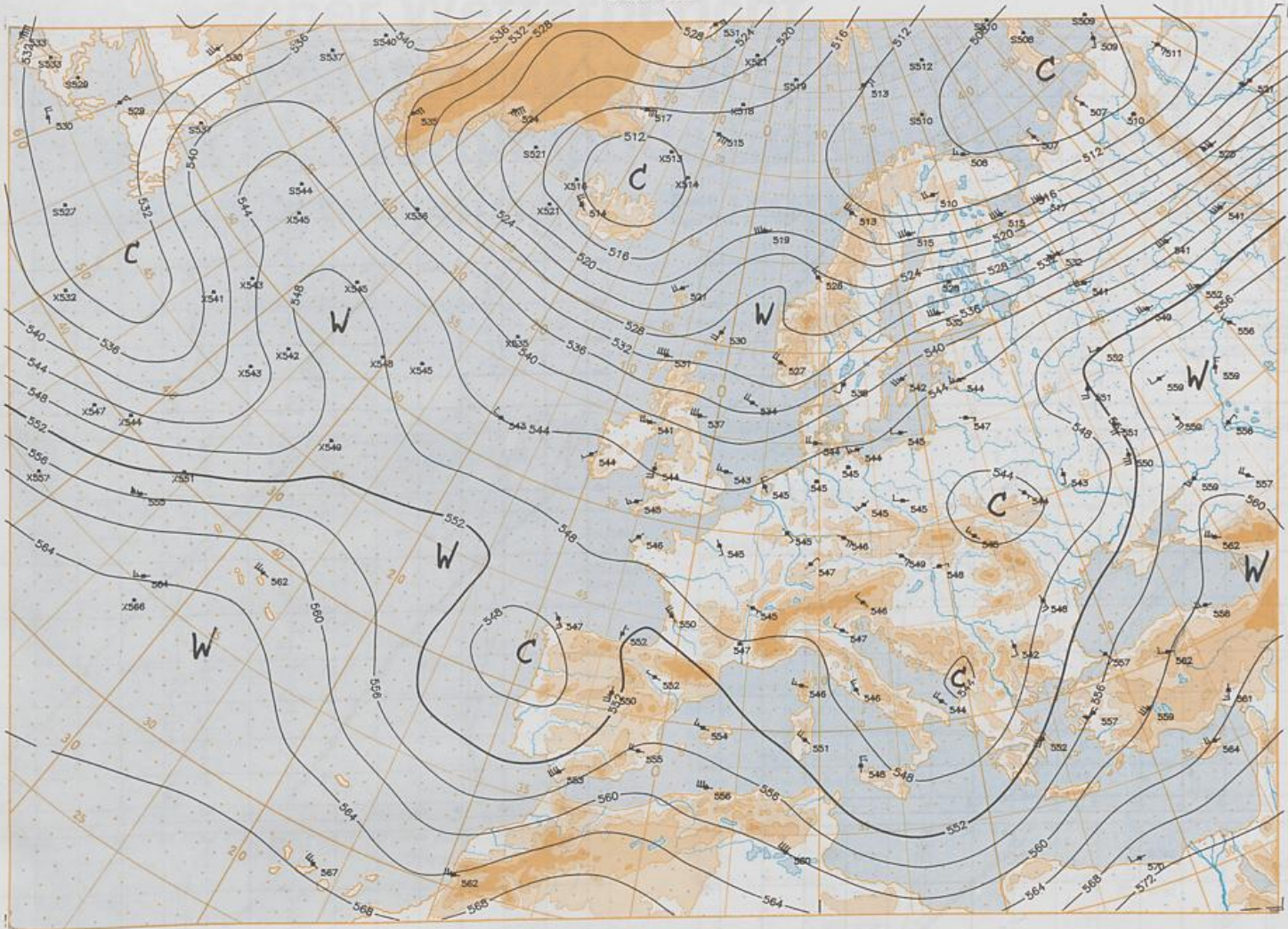
500/1000 hPa 12 UTC
