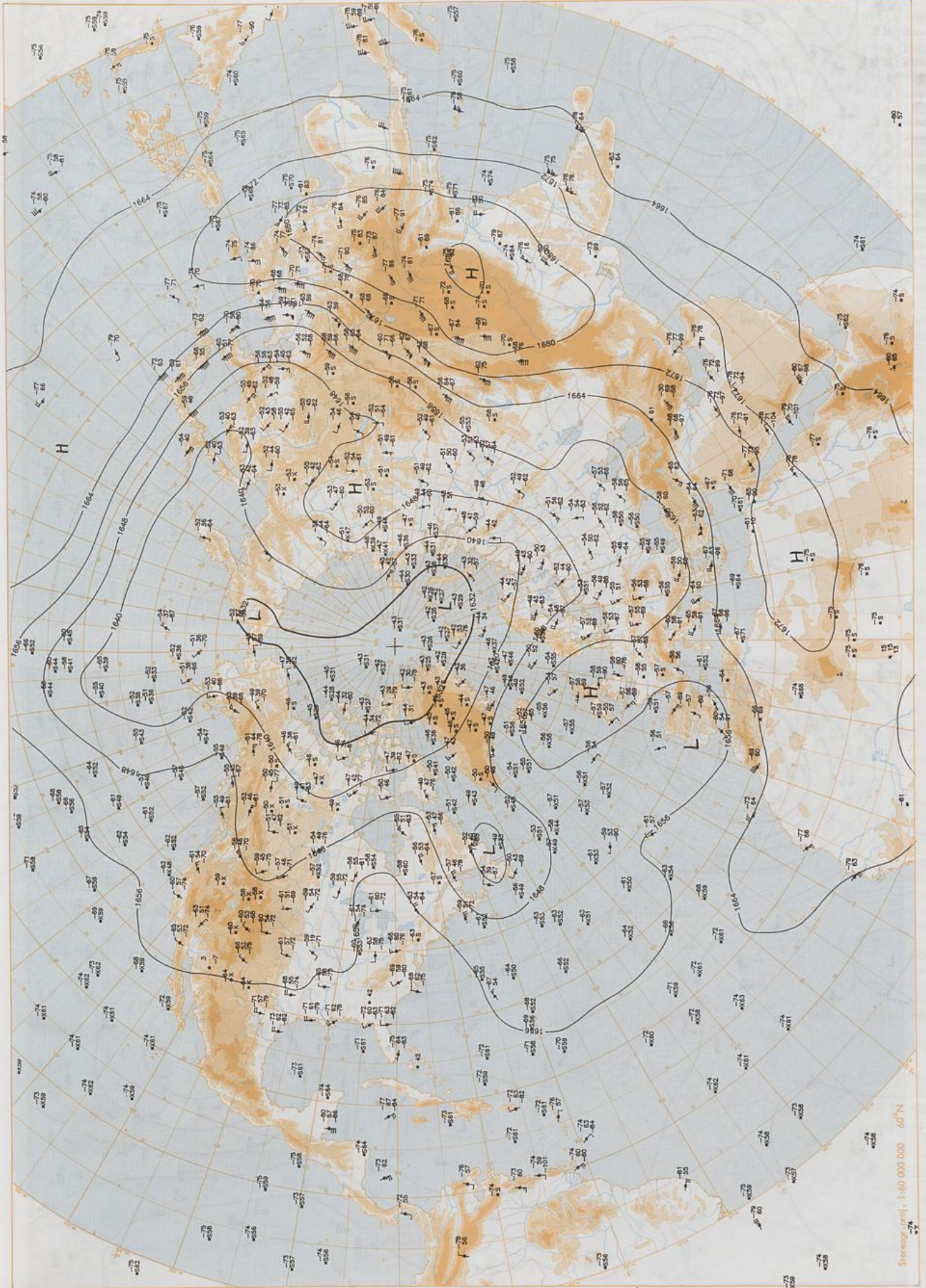
100 hPa 12 UTC
