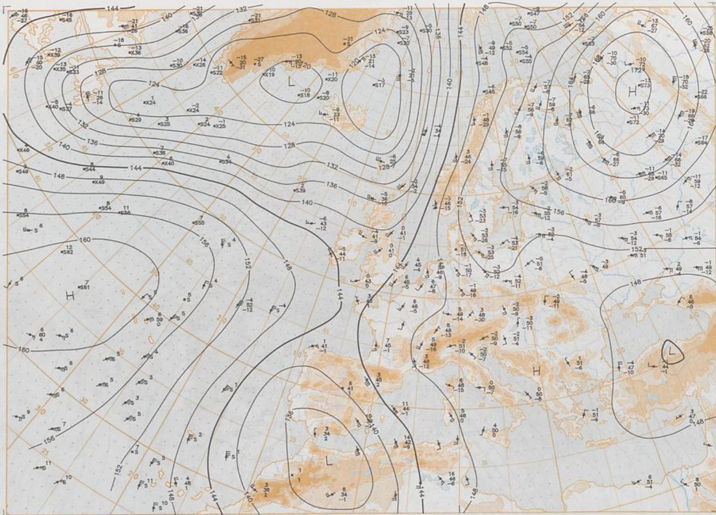
850 hPa 12 UTC
