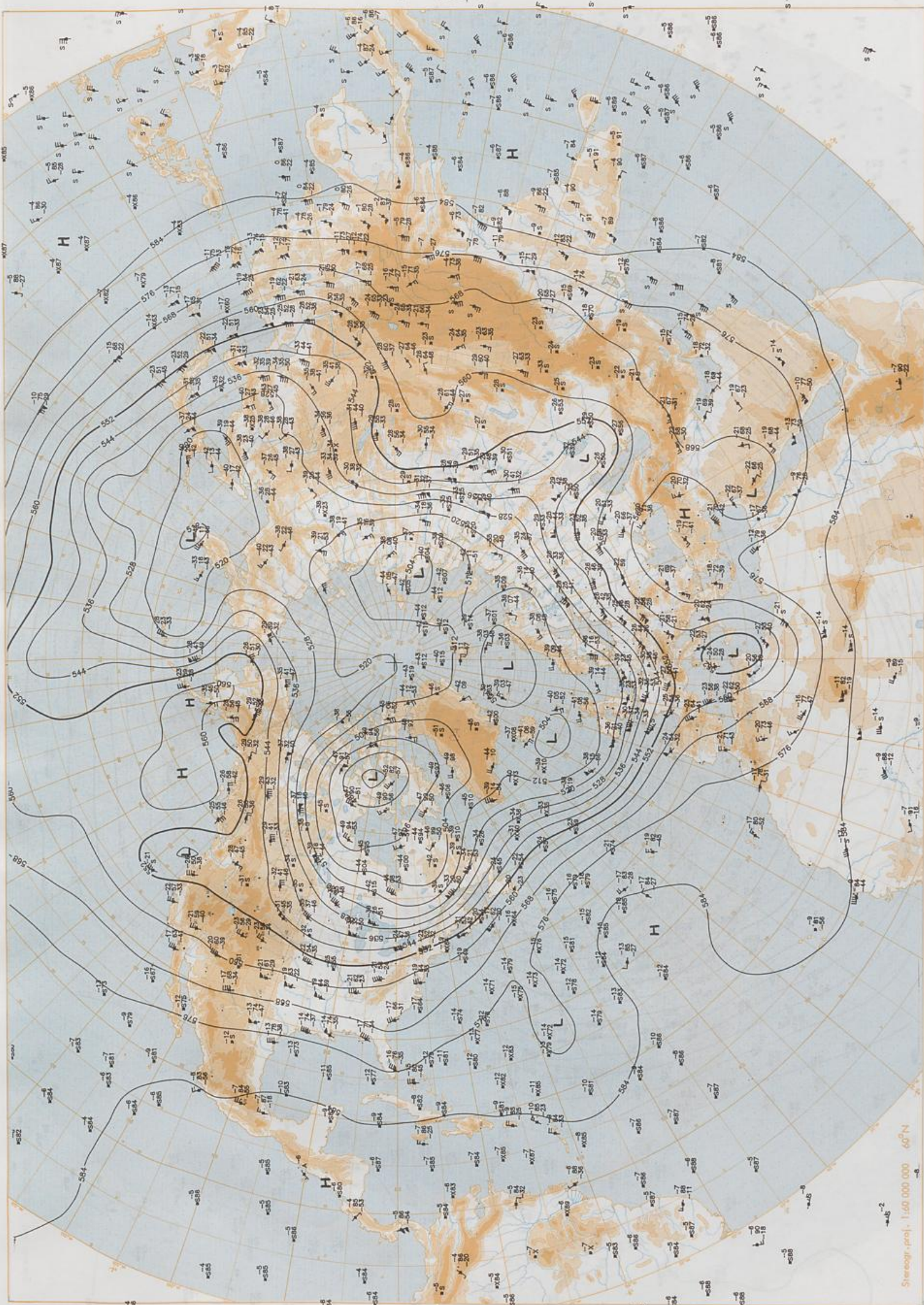
500 hPa 12 UTC
