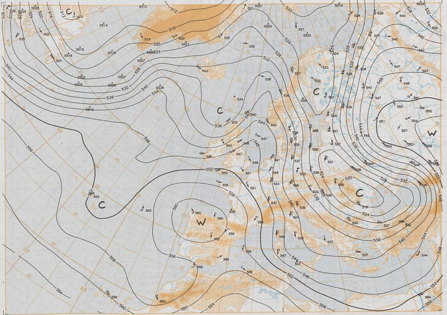
500/1000 hPa 12 UTC
