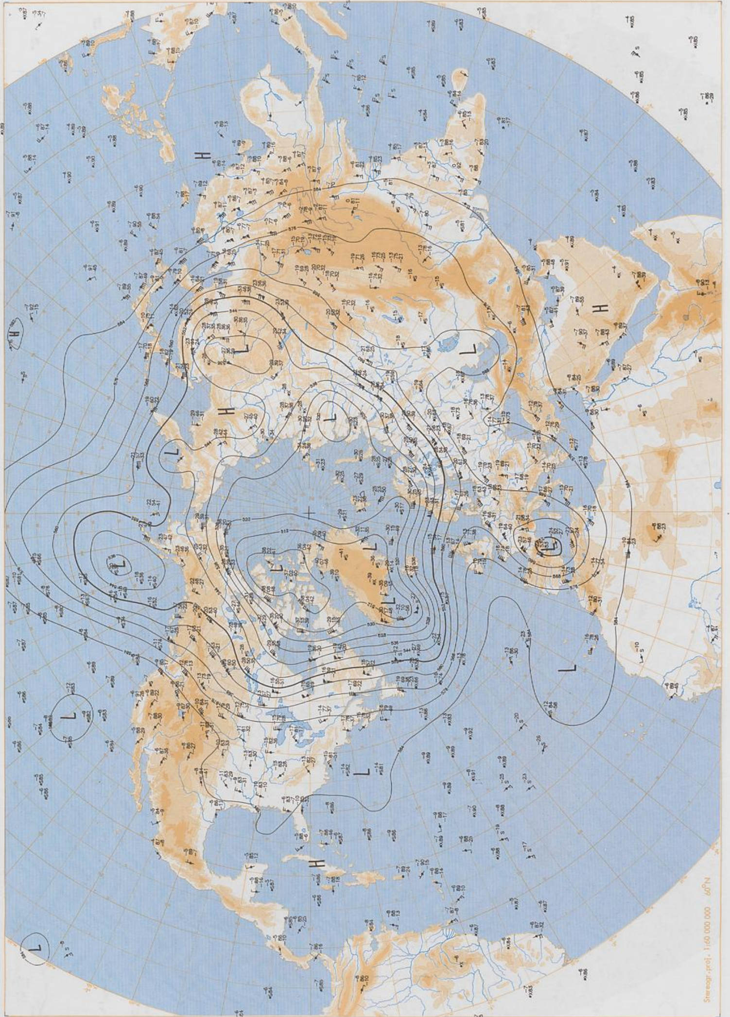
500 hPa 12 UTC
