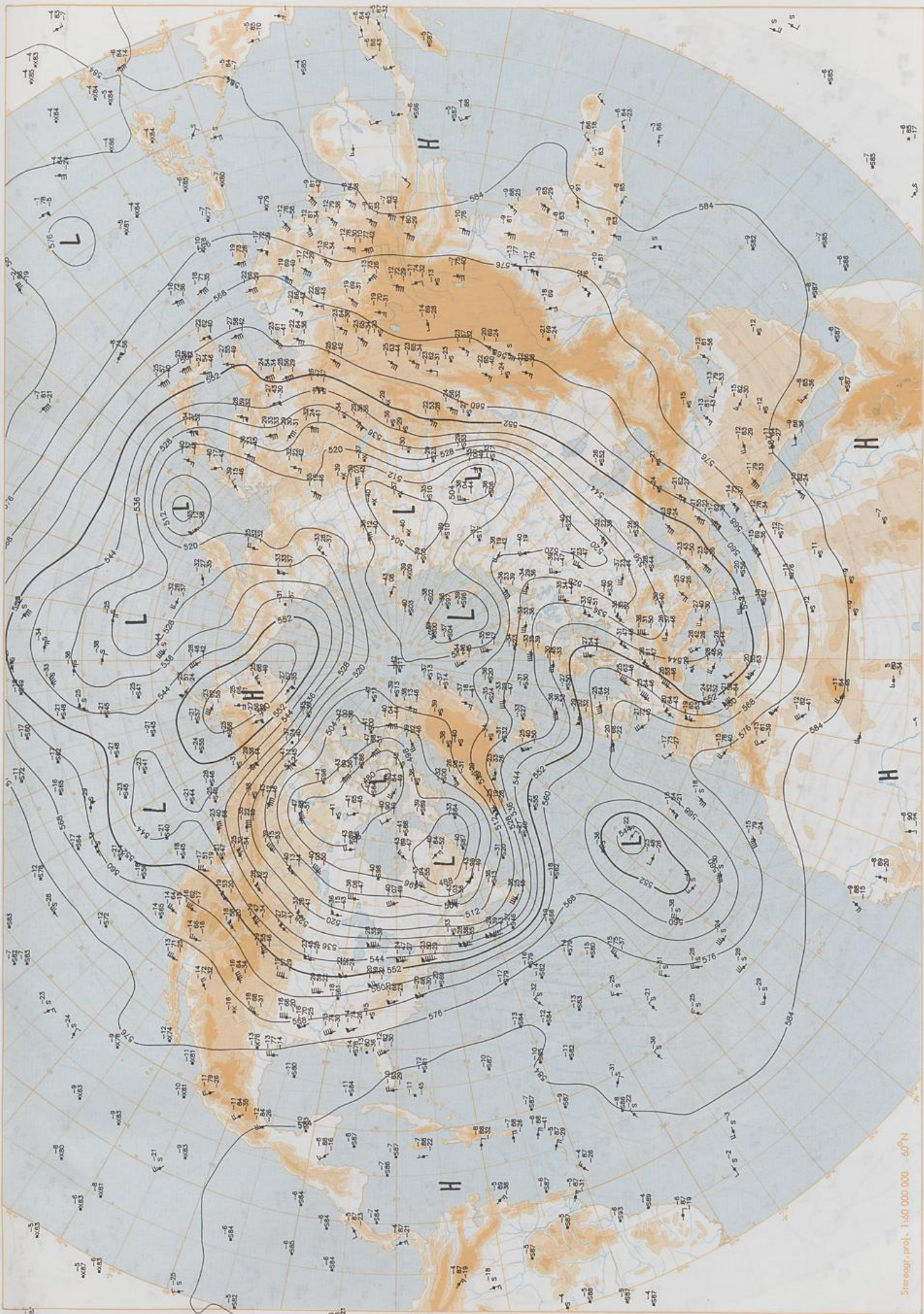
500 hPa 12 UTC
