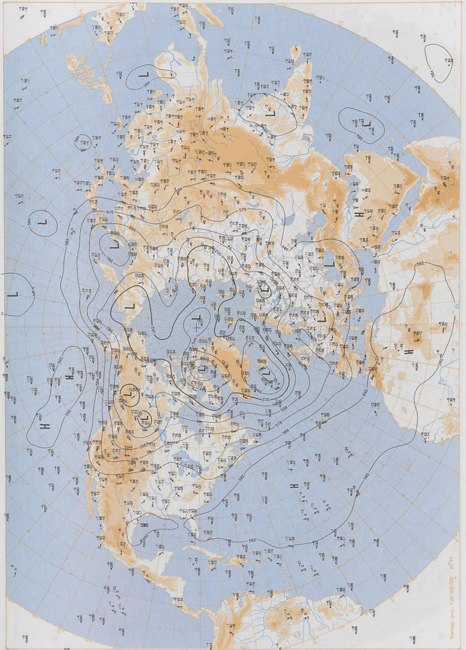
500 hPa 12 UTC
