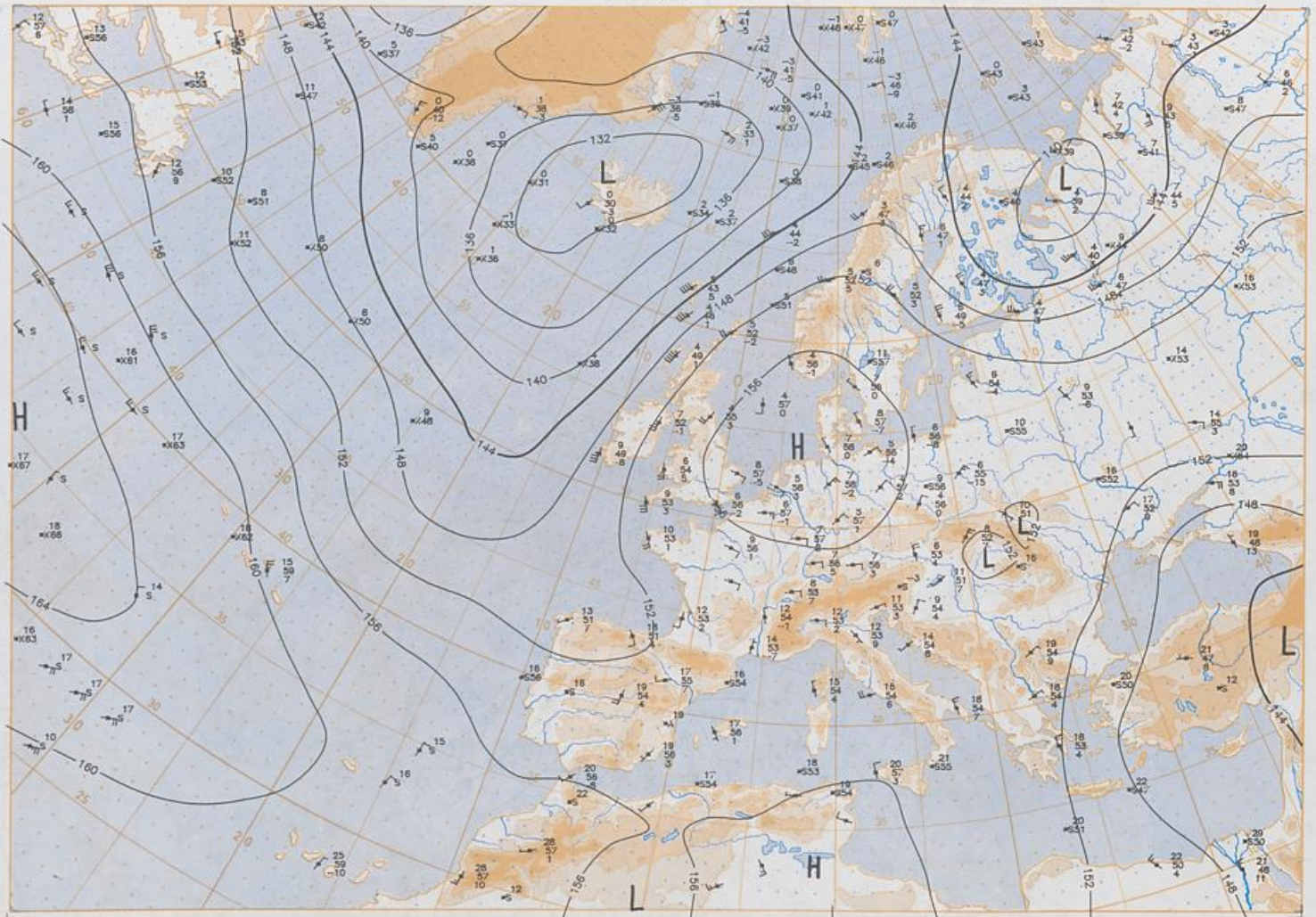
850 hPa 12 UTC
