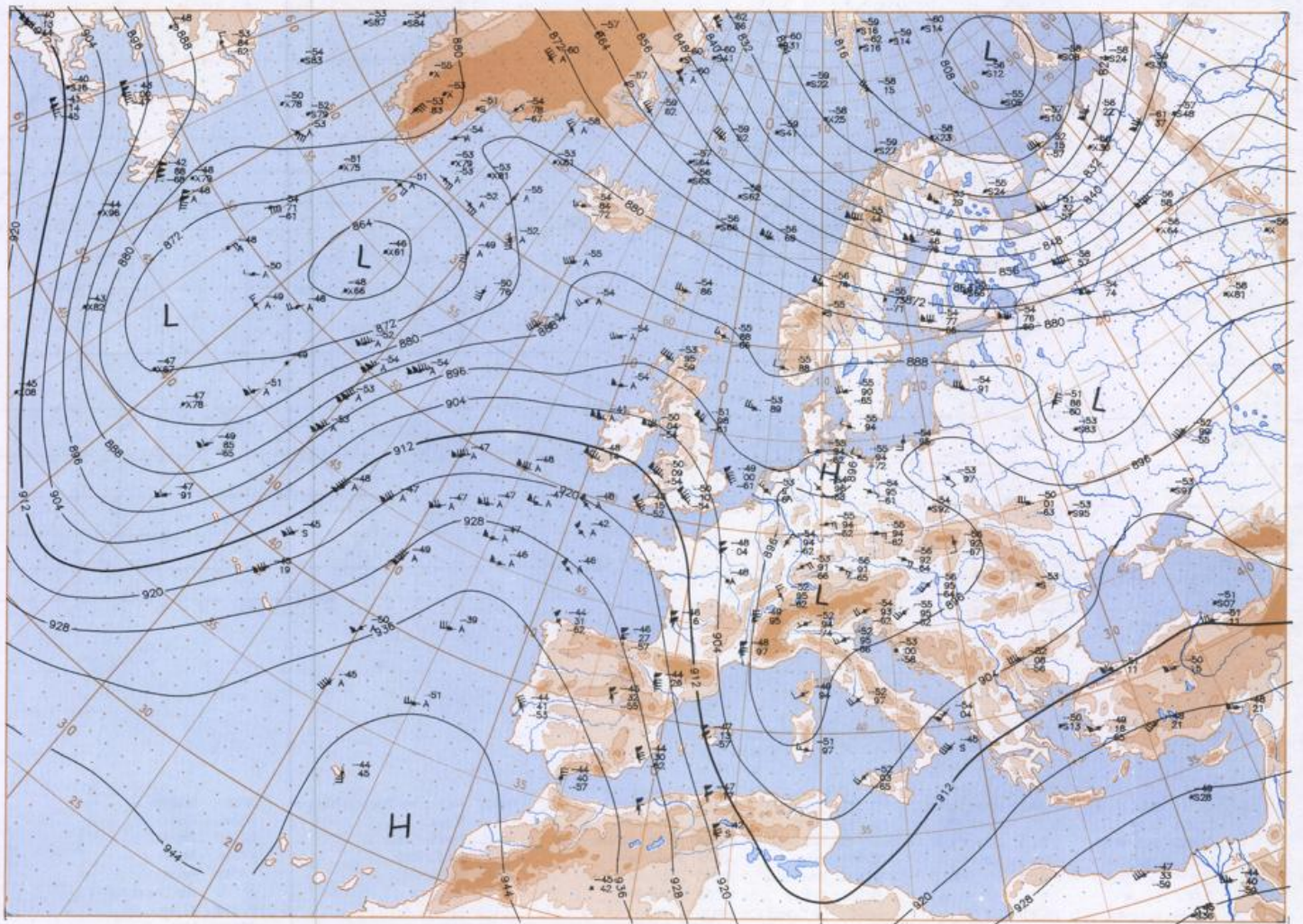
300 hPa 18 UTC
