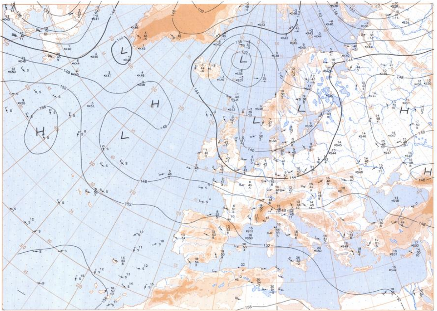
850 hPa 12 UTC
