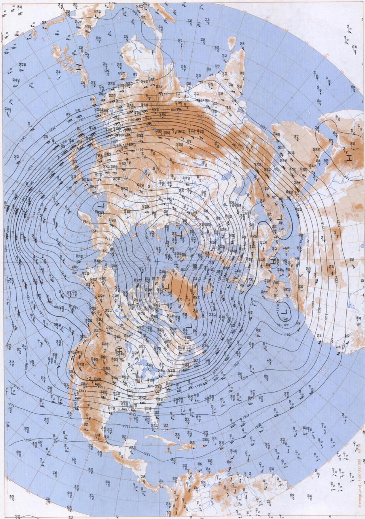
200 hPa 12 UTC
