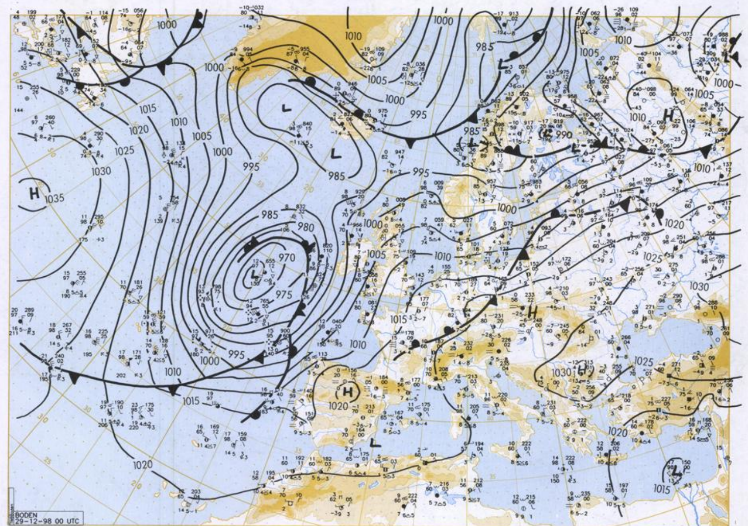
BODEN 29-12-98 00 UTC Stereogr. proj. 1:30 000 000 60°N Surface chart 00 UTC
