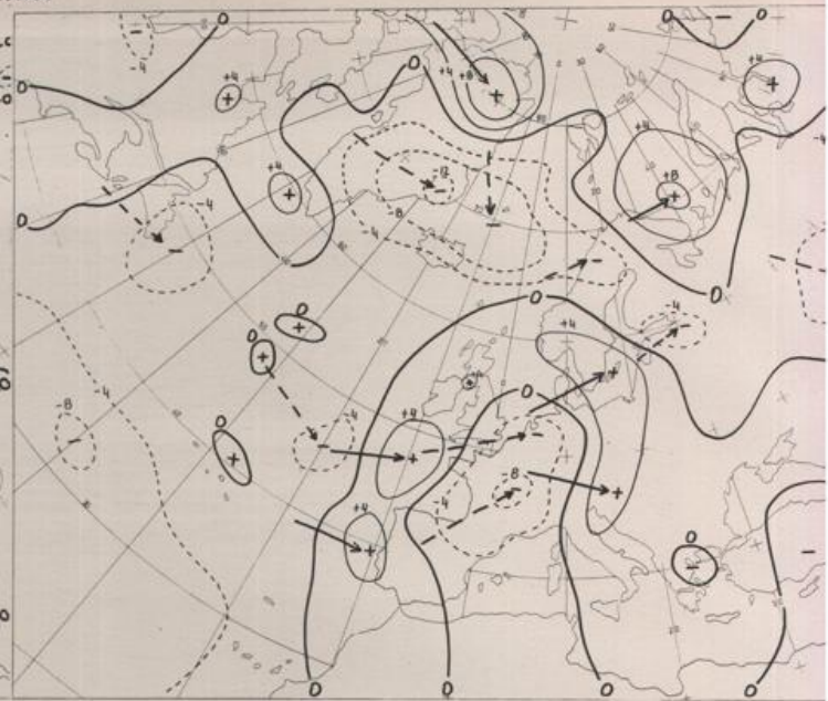
24 hr thickness change 00 GMT
