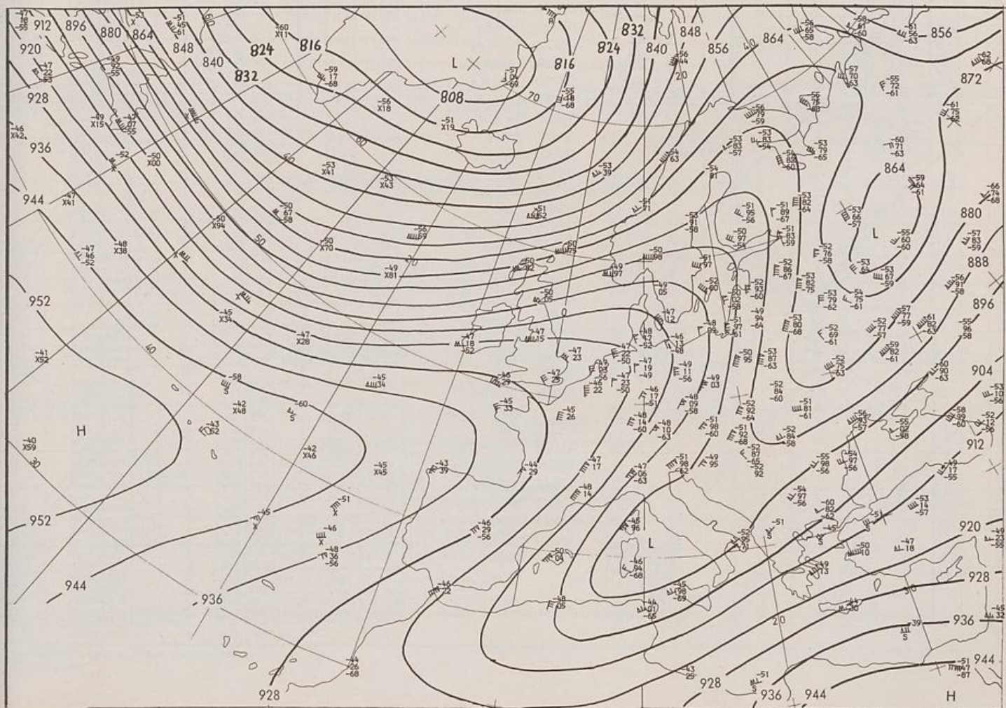
300 hPa 00 GMT
