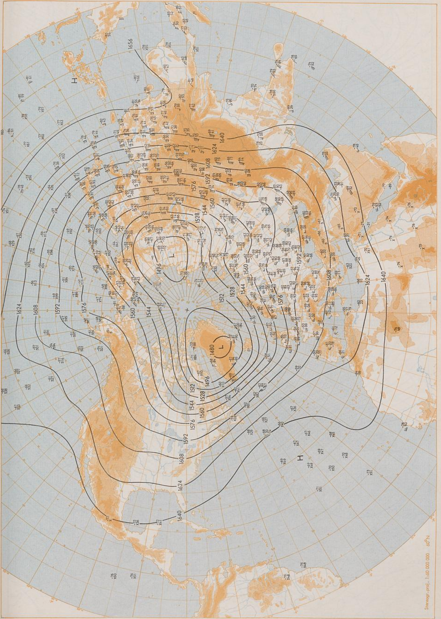
100 hPa 00 GMT
