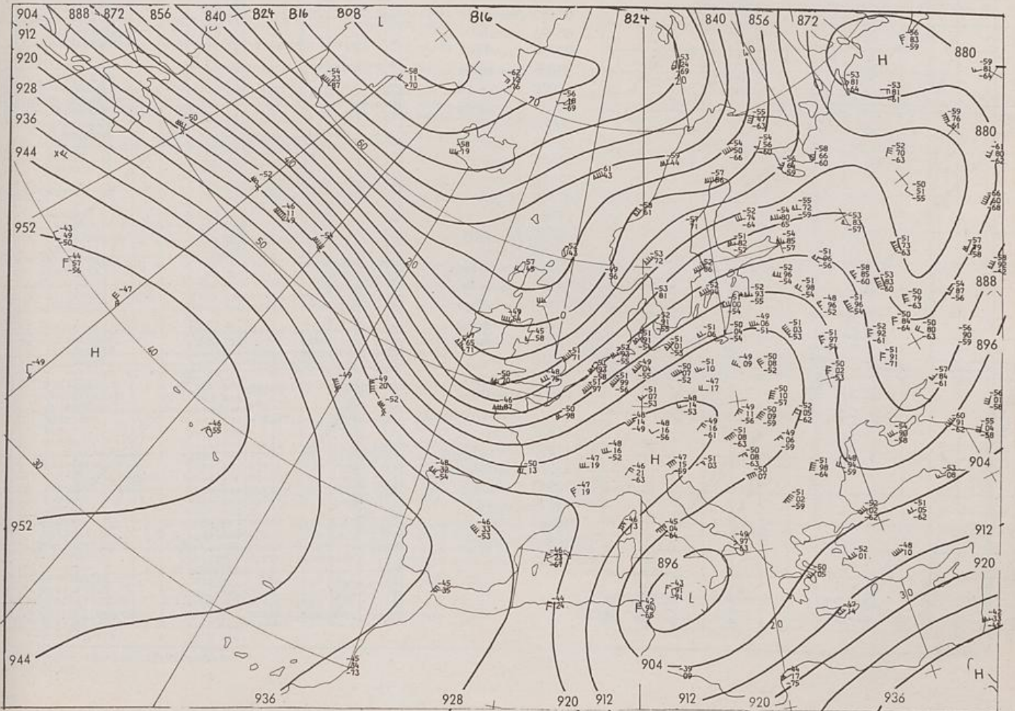
300 hPa 00 GMT
