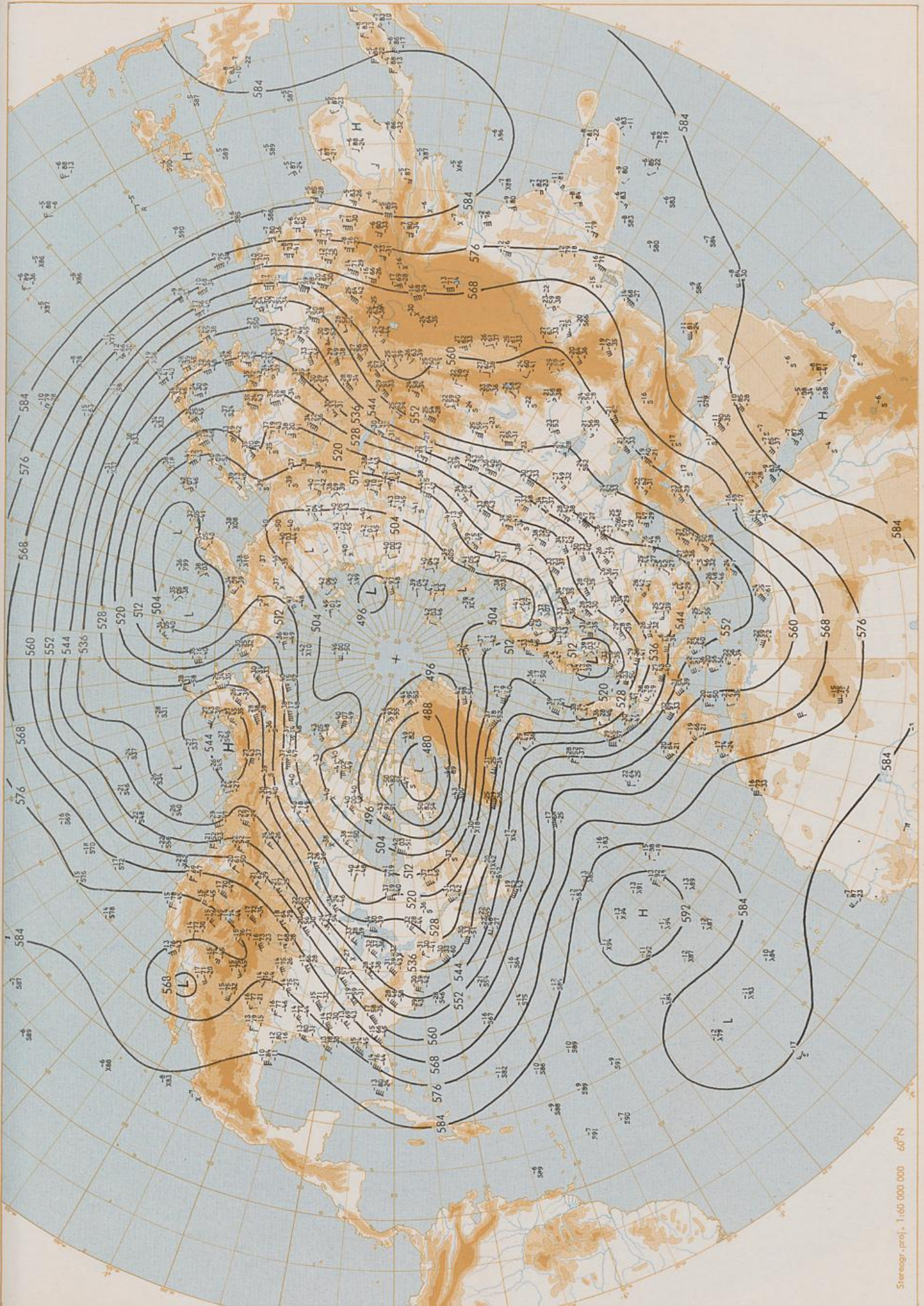
500 hPa 00 GMT
