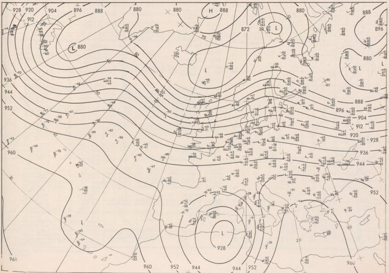
300 hPa 00 GMT
