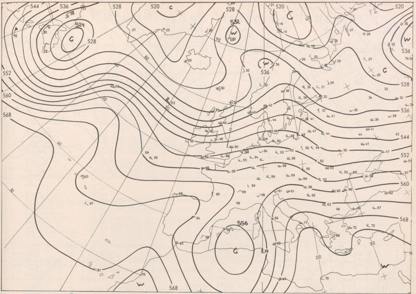
500/1000 hPa 00 GMT
