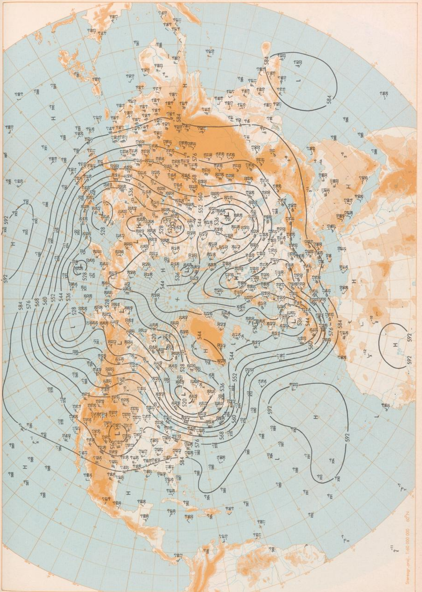
500 hPa 00 GMT
