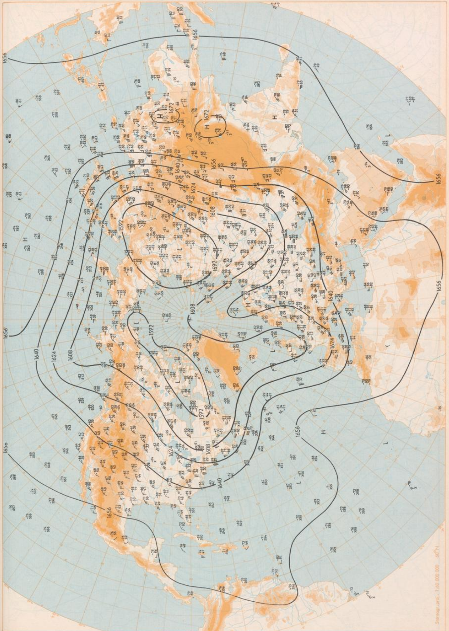
100 hPa CO GMT
