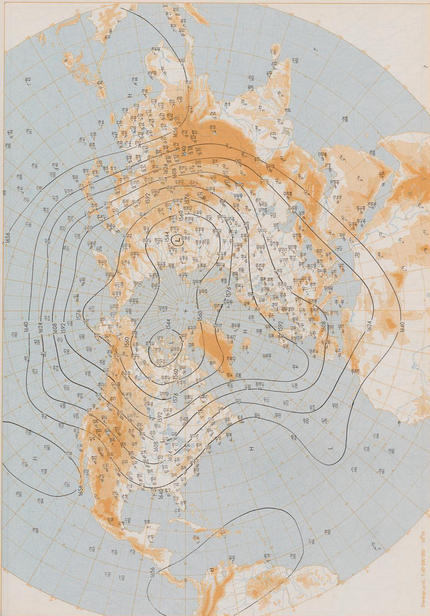
100 hPa 00 GMT
