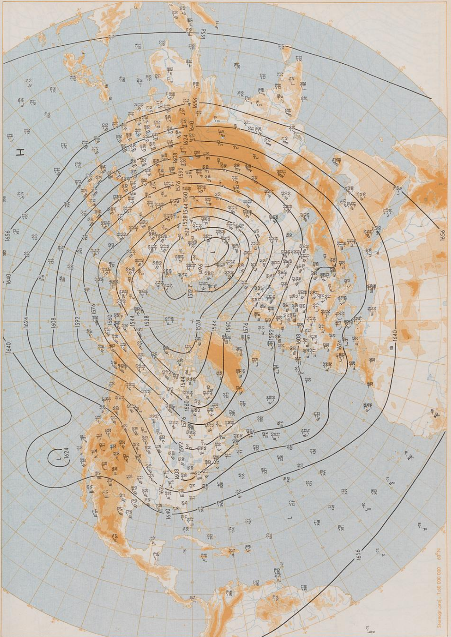
100 hPa 00 GMT
