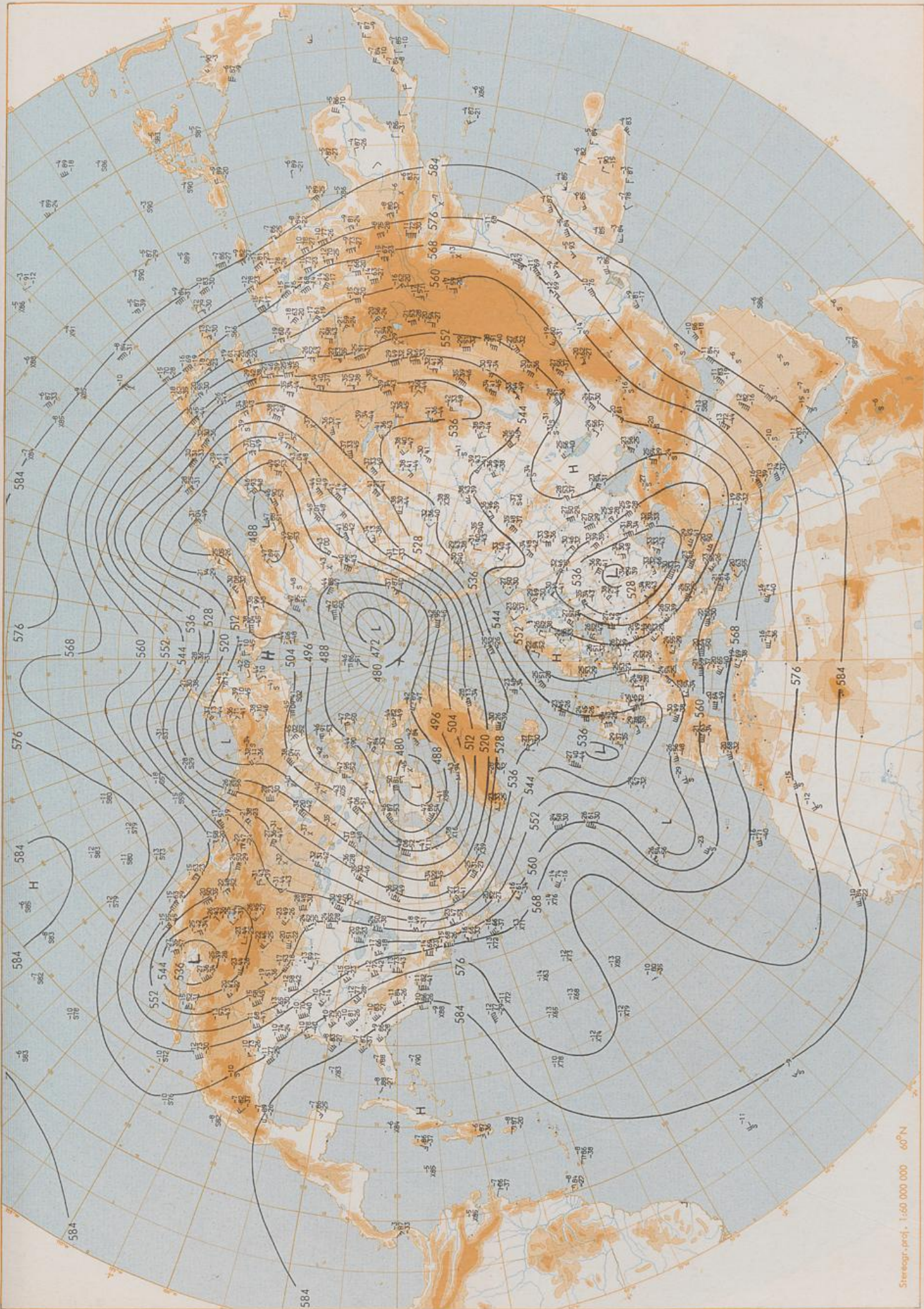
500 hPa 00 GMT
