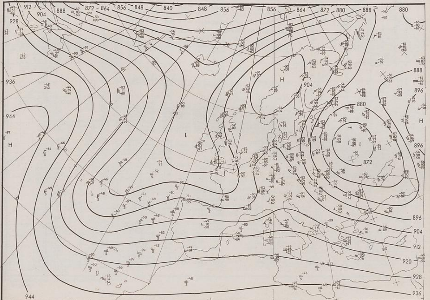
300 hPa 00 GMT
