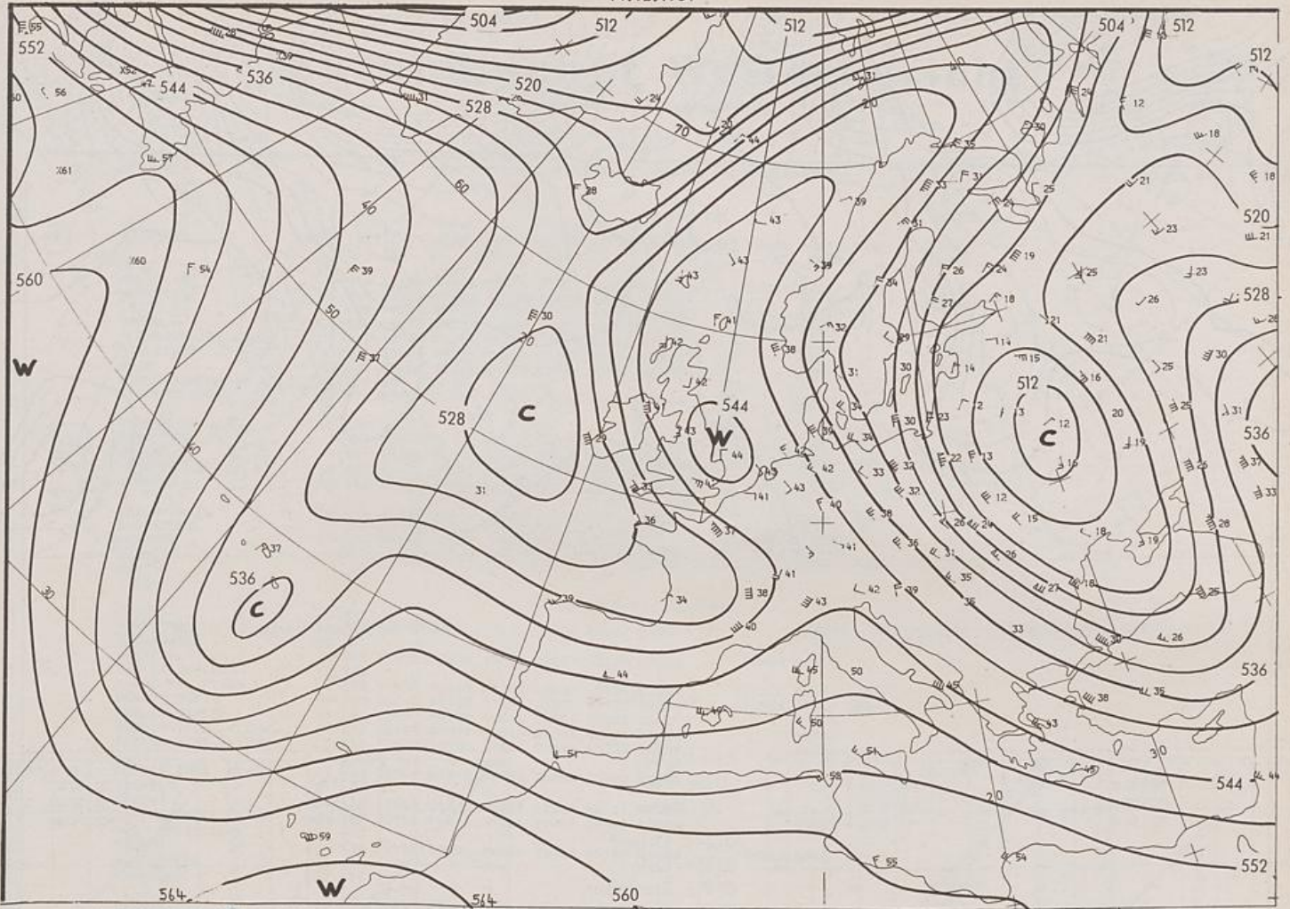
500/1000 hPa 00 GMT
