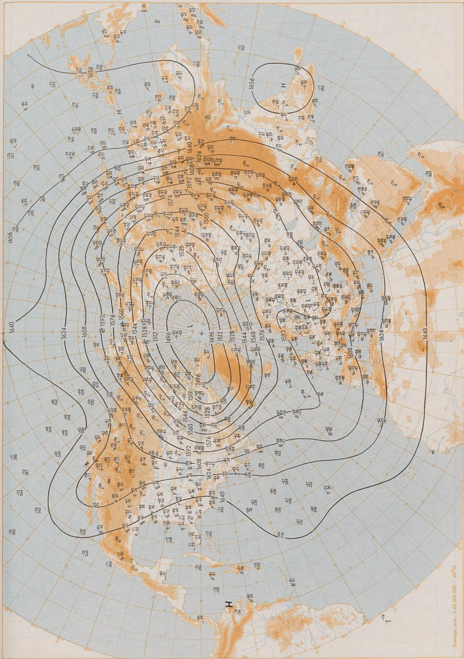
100 hPa 00 GMT
