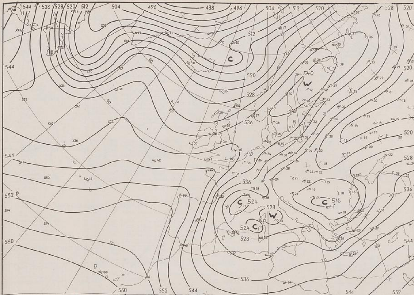
500/1000 hPa 00 GMT
