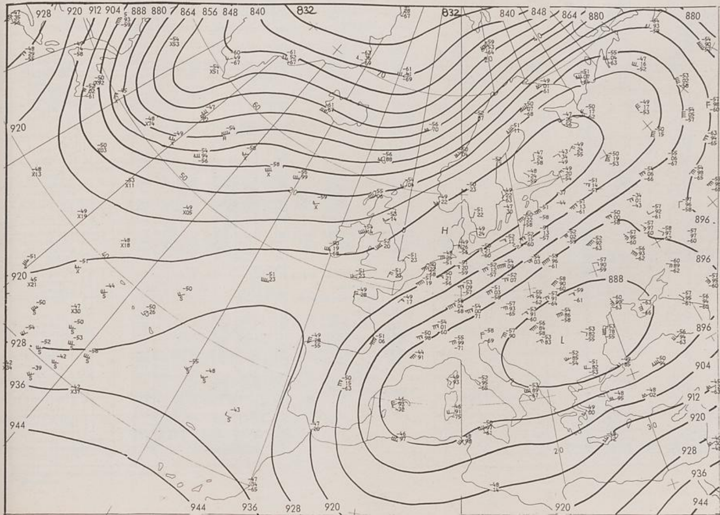
300 hPa 00 GMT
