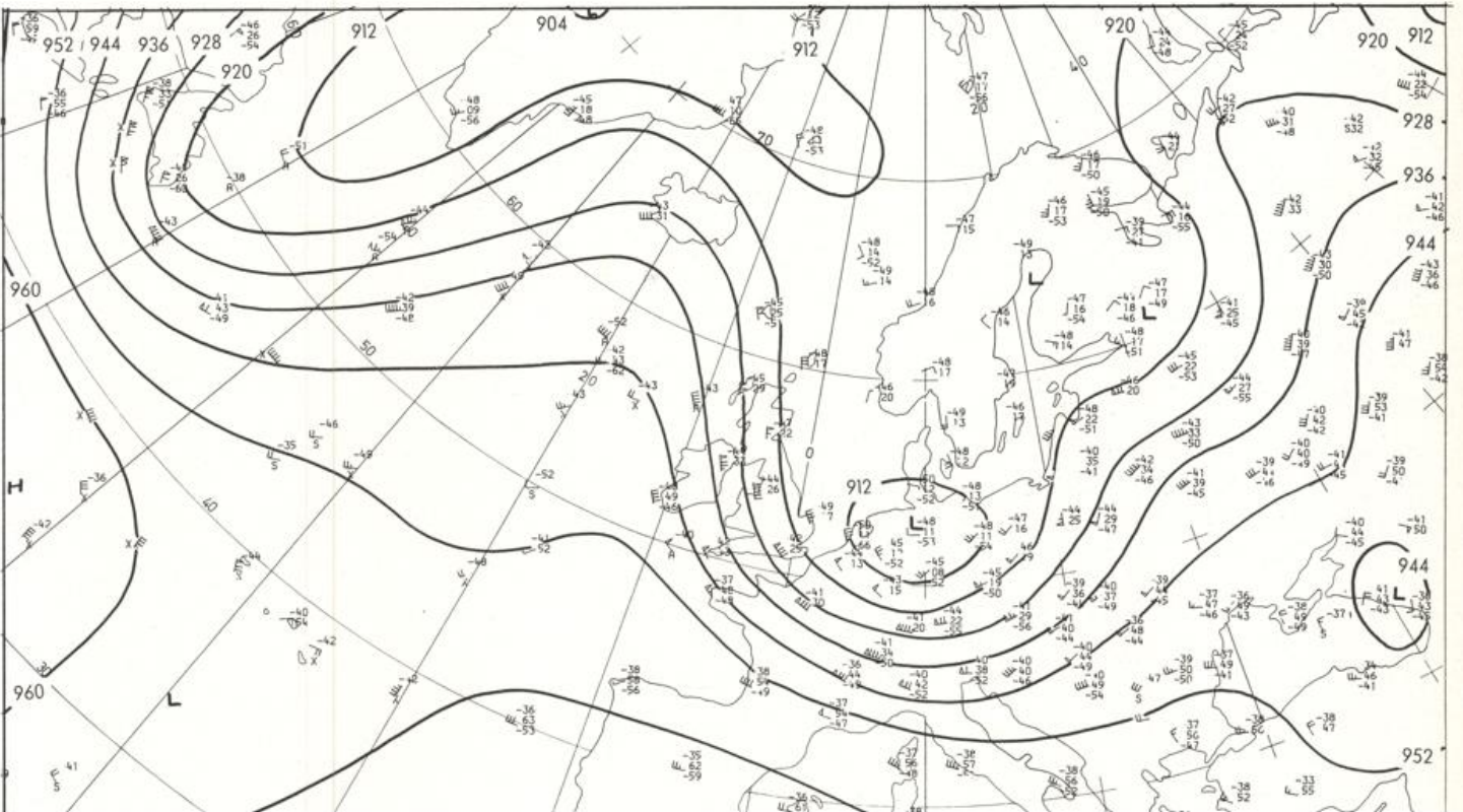
500/1000 hPa 00 GMT
