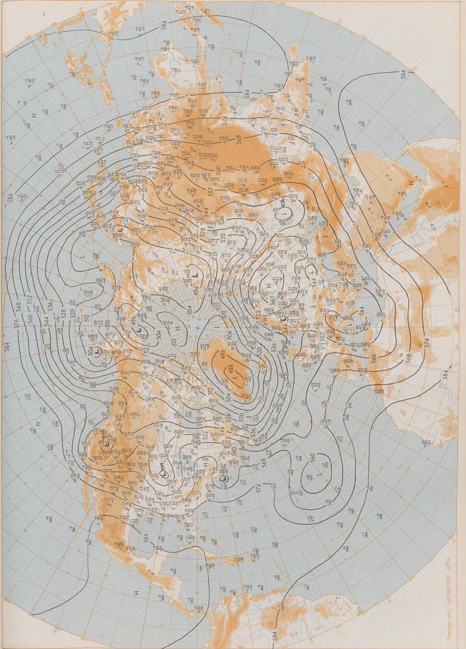
500 hPa 00 GMT
