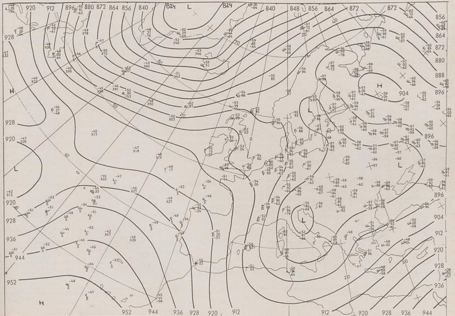
300 hPa 00 GMT
