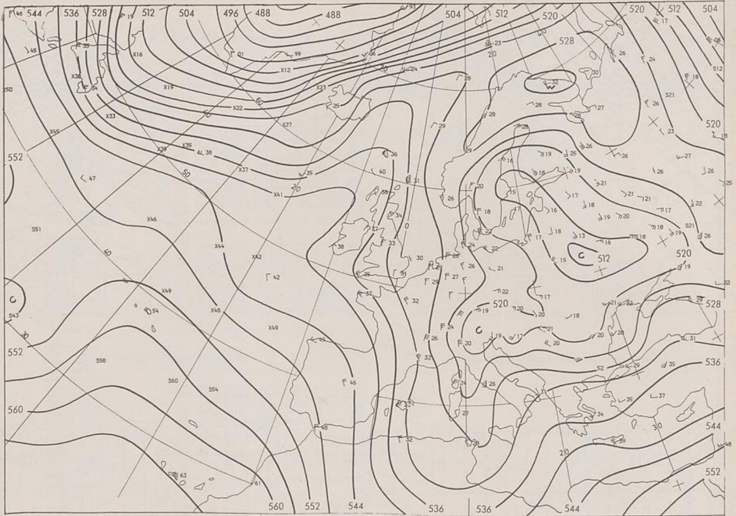
500/1000 hPa 00 GMT
