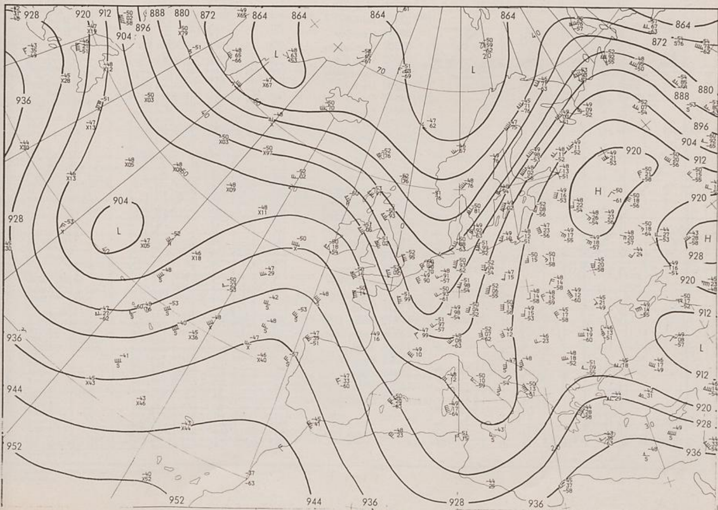
300 hPa 00 GMT
