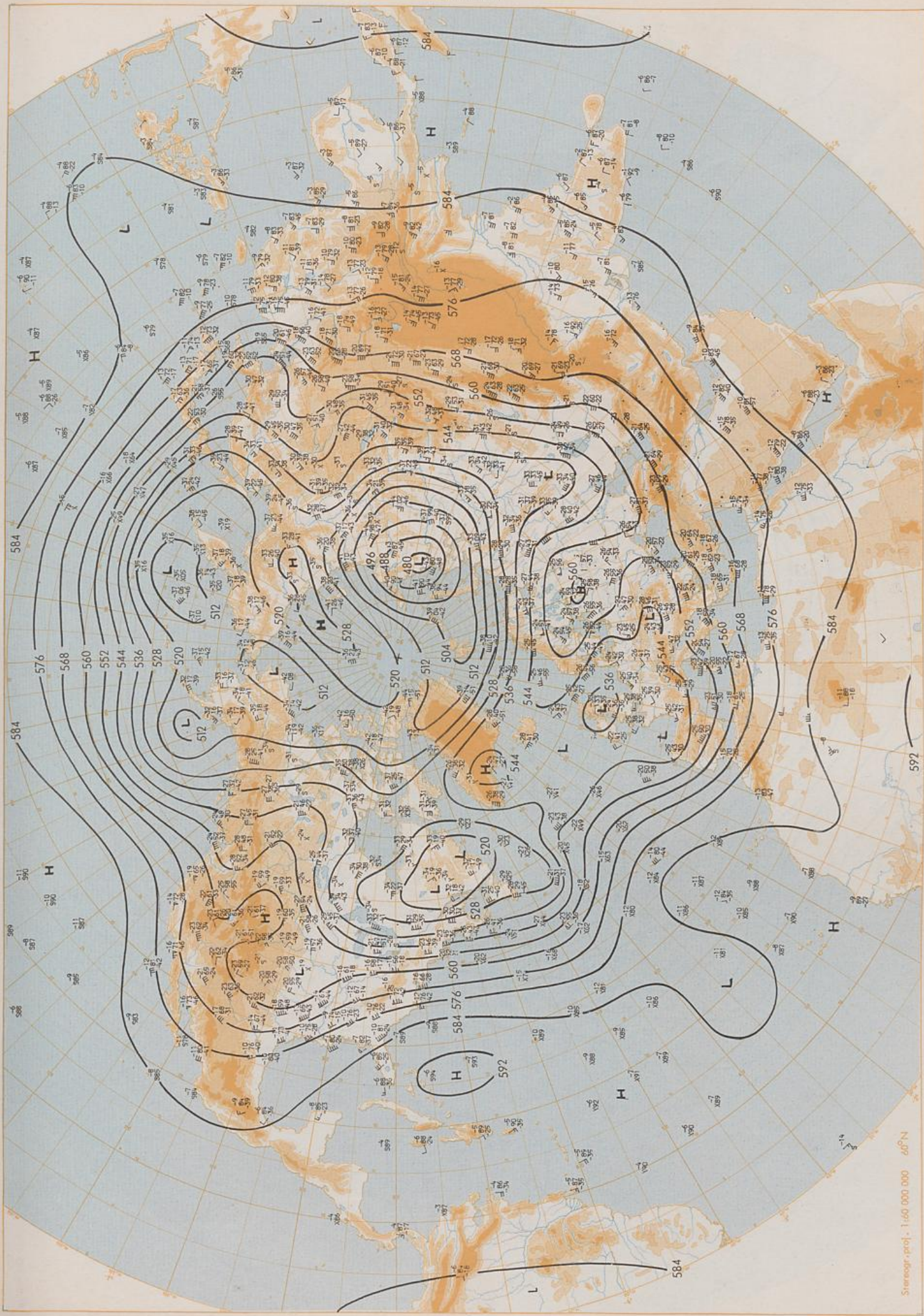
500 hPa 00 GMT
