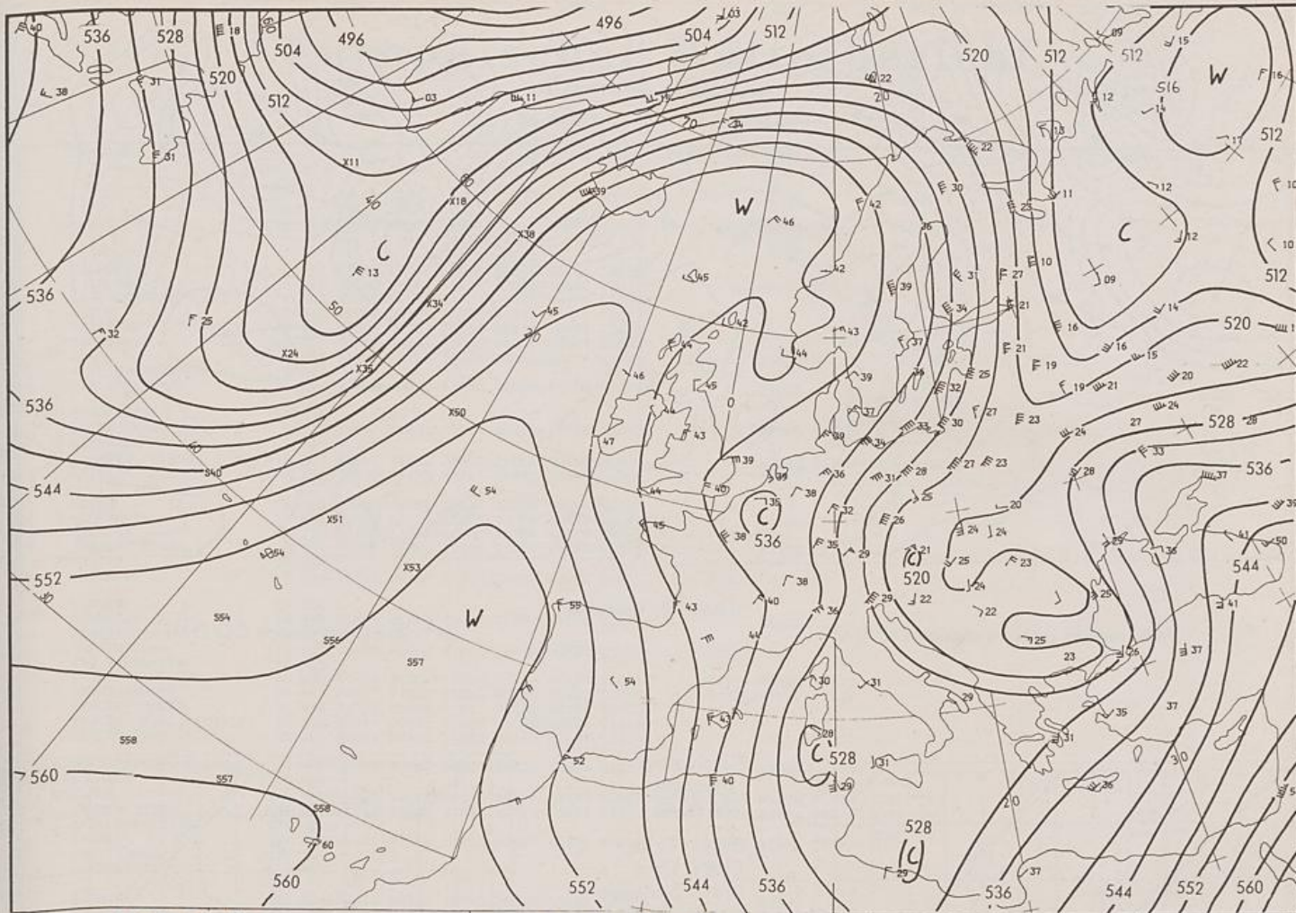
500/1000 hPa 00 GMT
