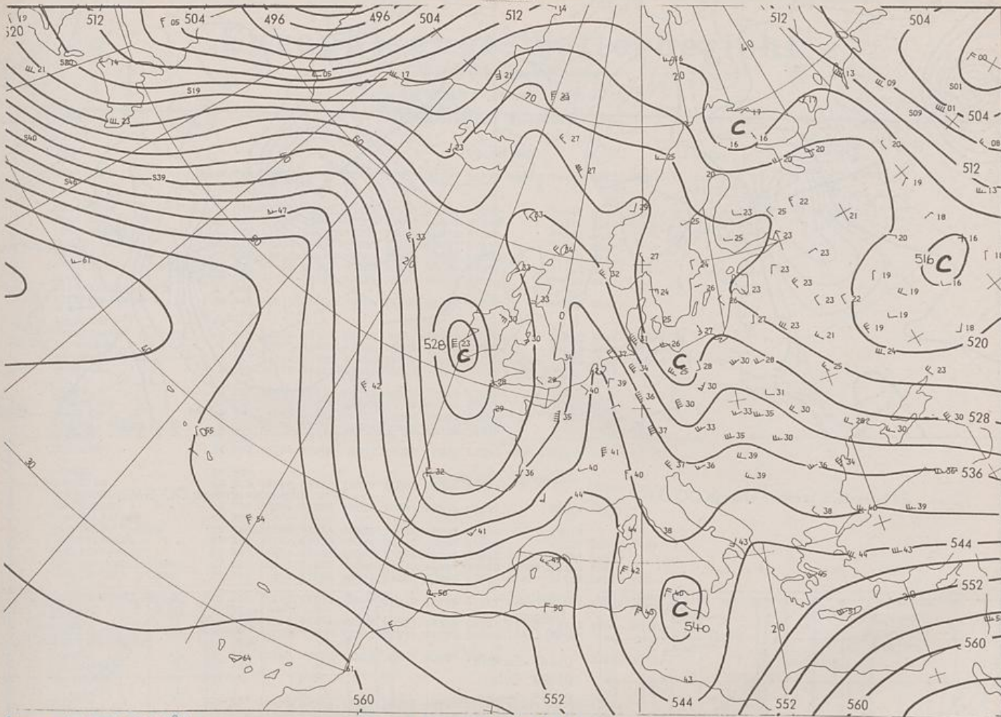
500/1000 hPa 00 GMT
