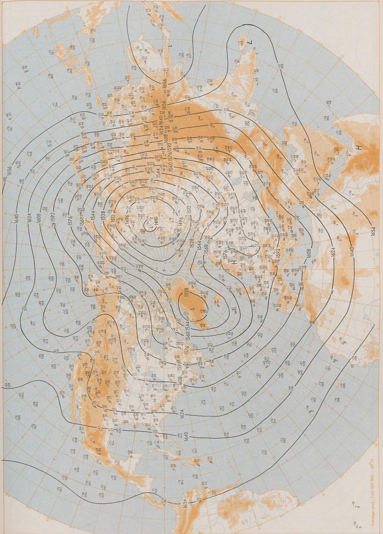
100 hPa 00 GMT
