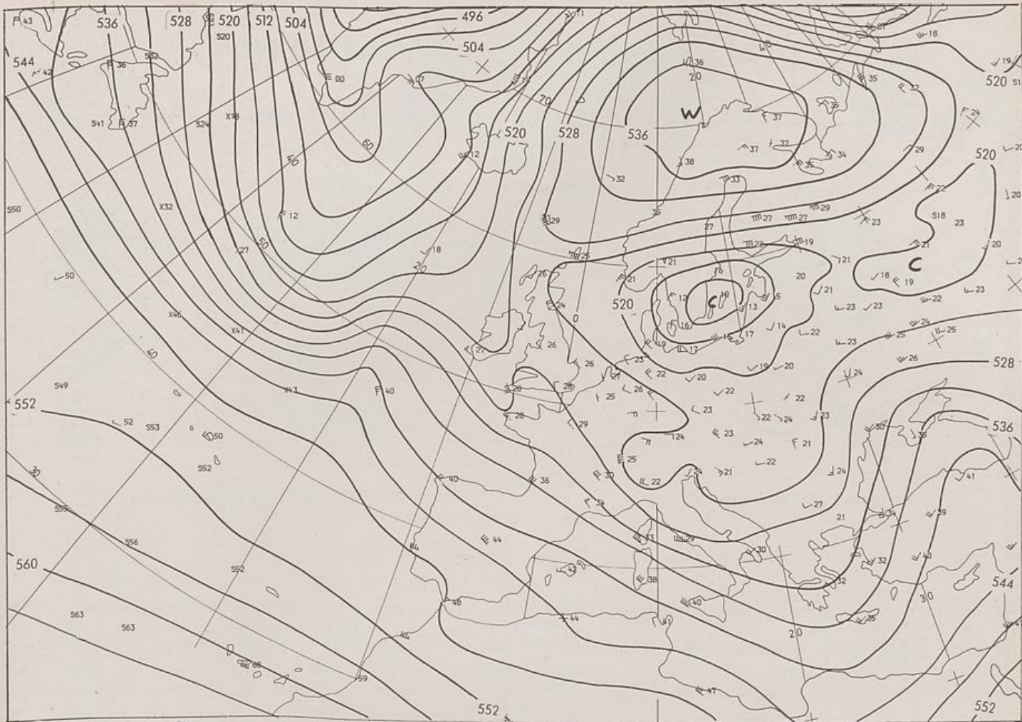
500/1000 hPa 00 GMT
