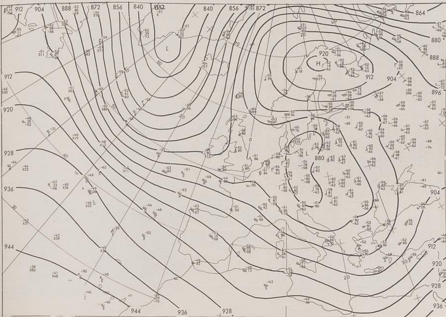
300 hPa 00 GMT
