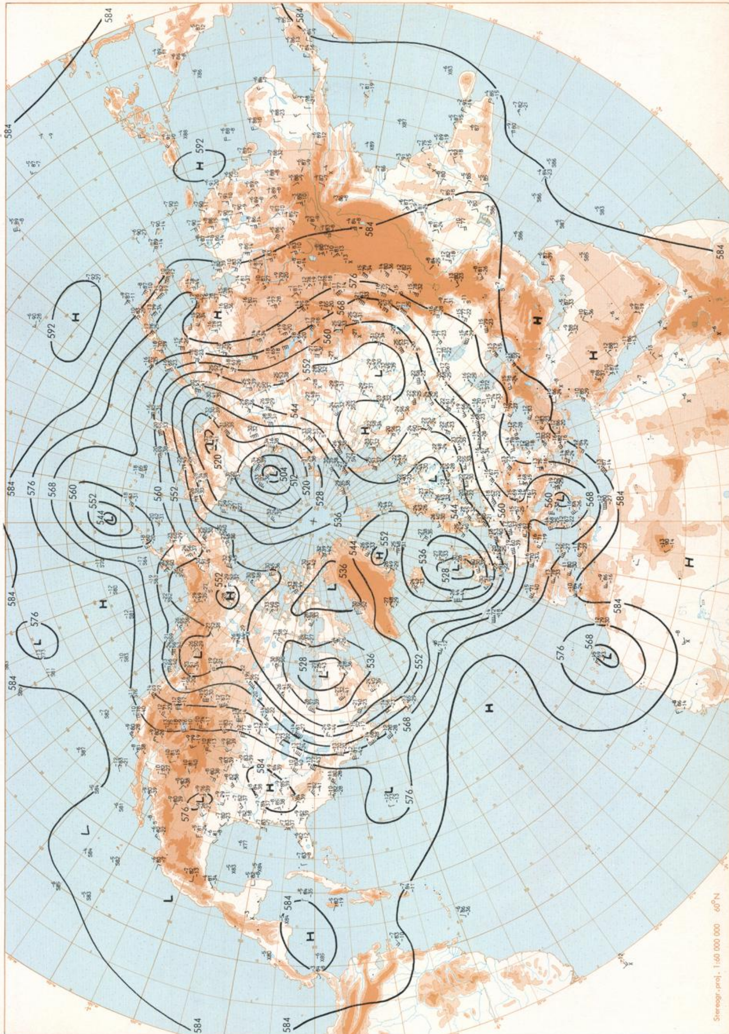
500 hPa 00 GMT
