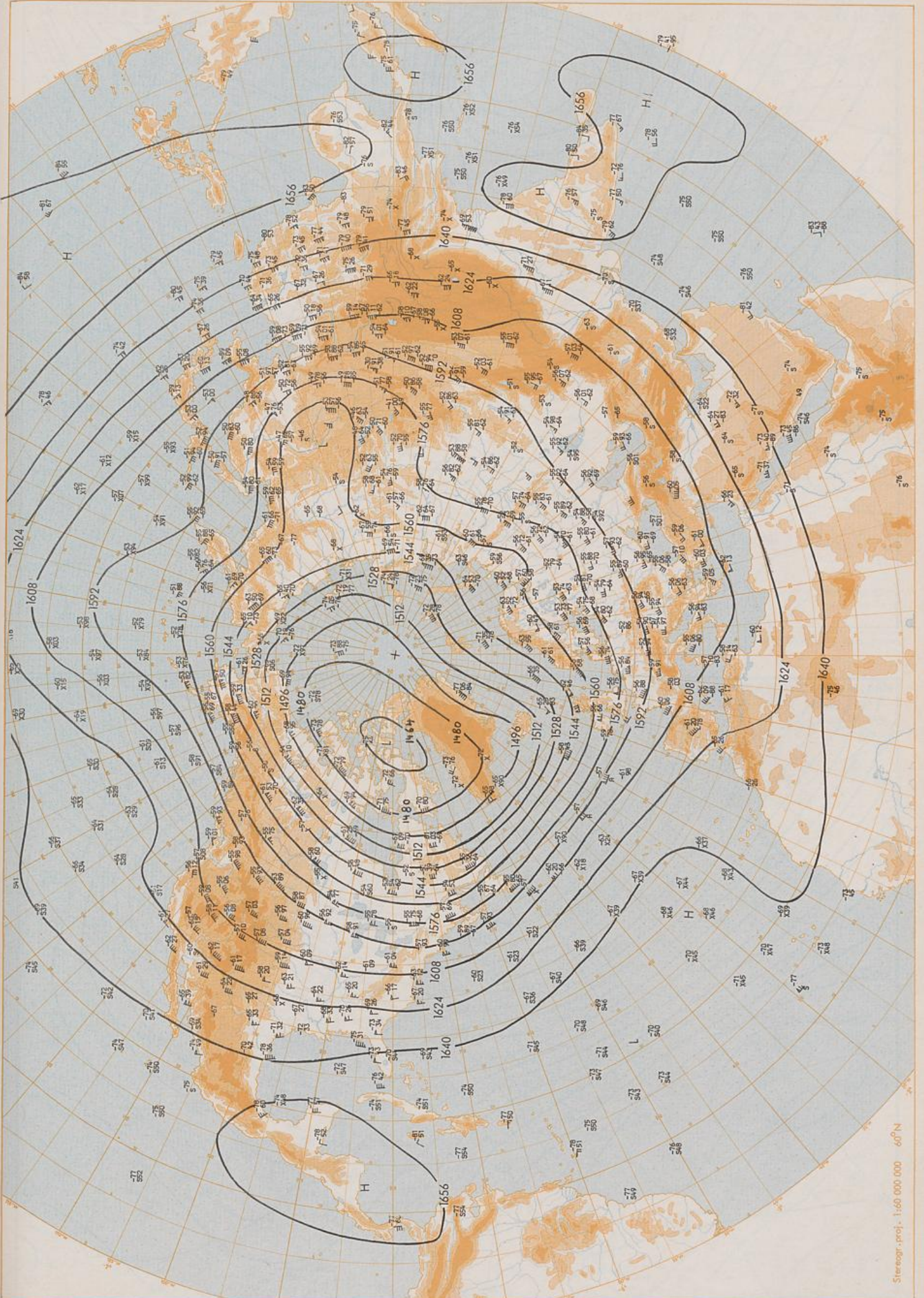
100 hPa 00 GMT
