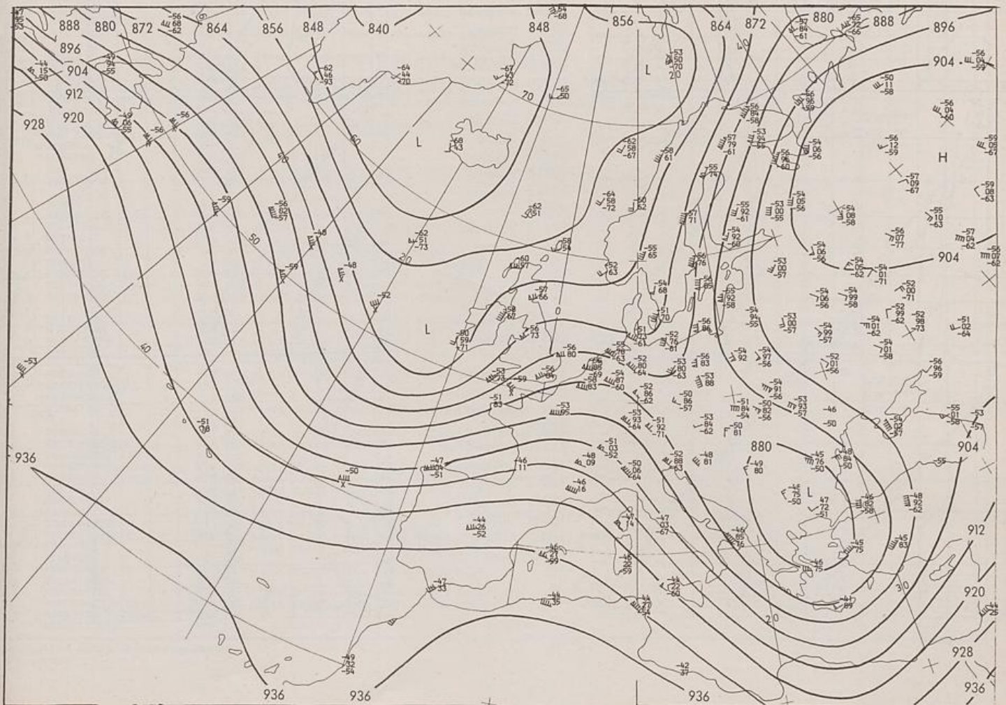
500/1000 hPa 00 GMT
