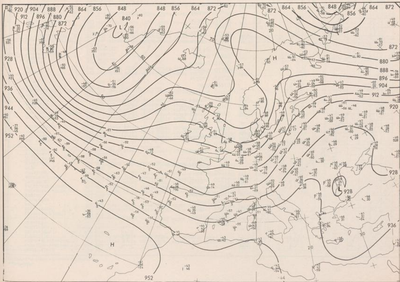
300 hPa 00 GMT
