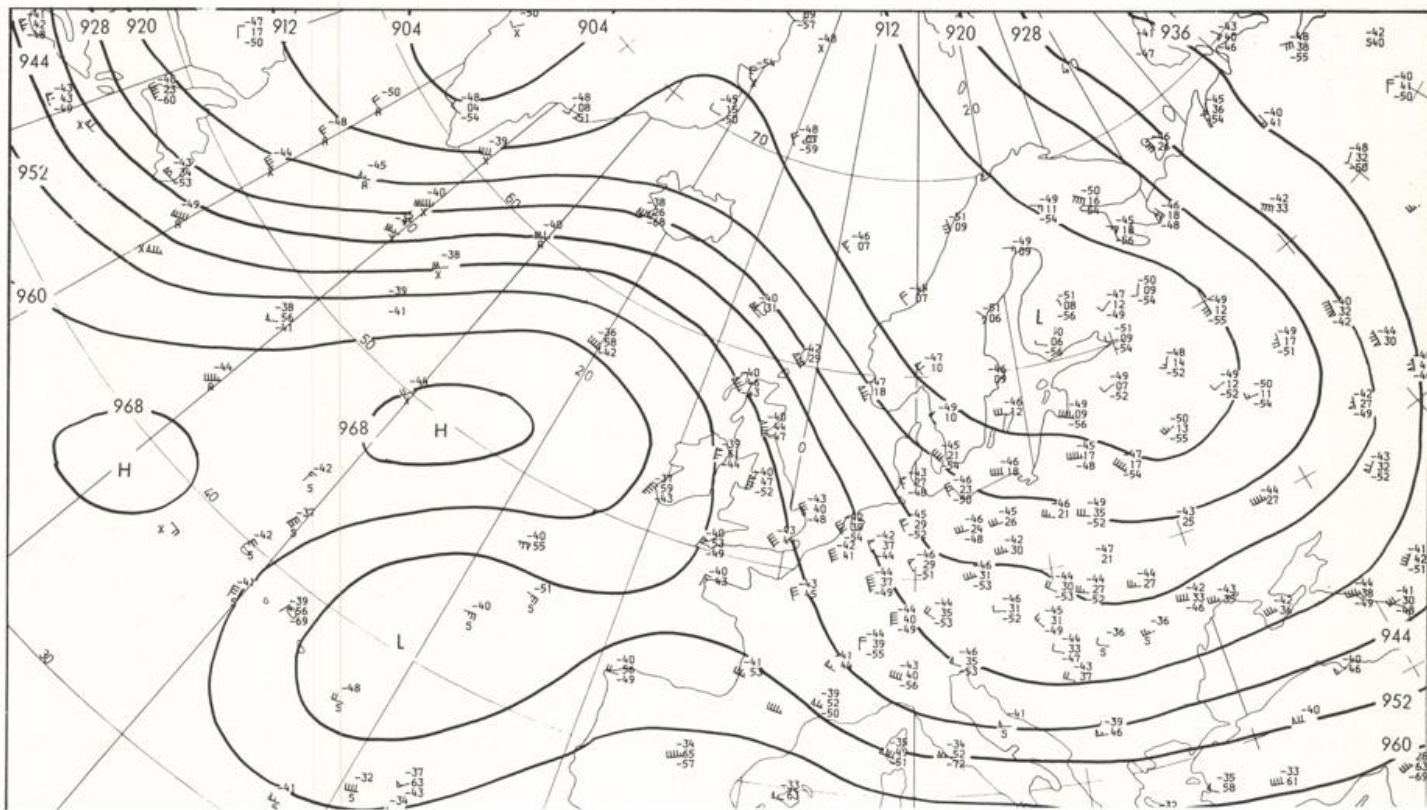
500/1000 hPa 00 GMT
