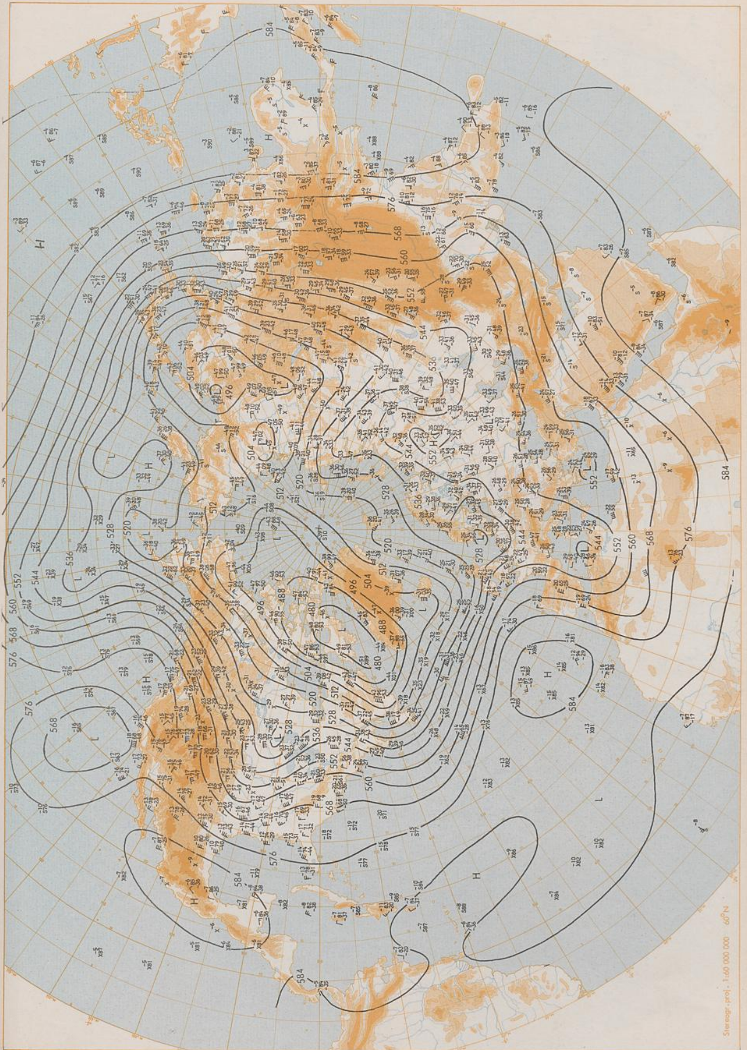
500 hPa 00 GMT
