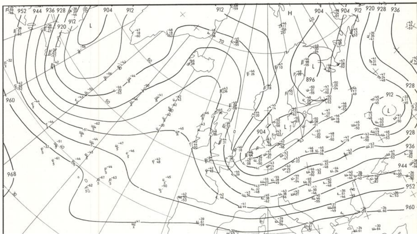
500/1000 hPa 00 GMT
