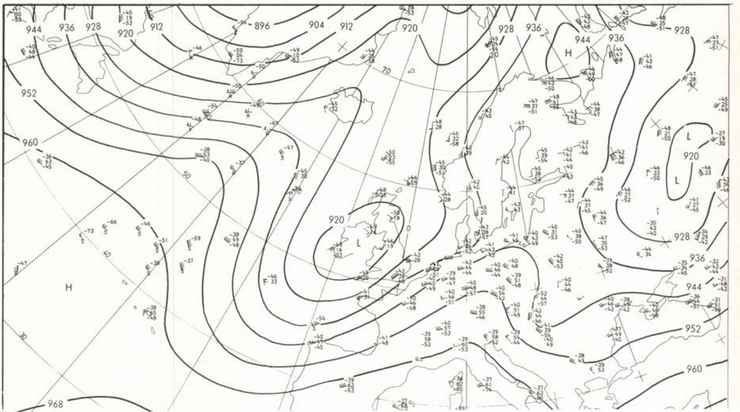
500/1000 hPa 00 GMT
