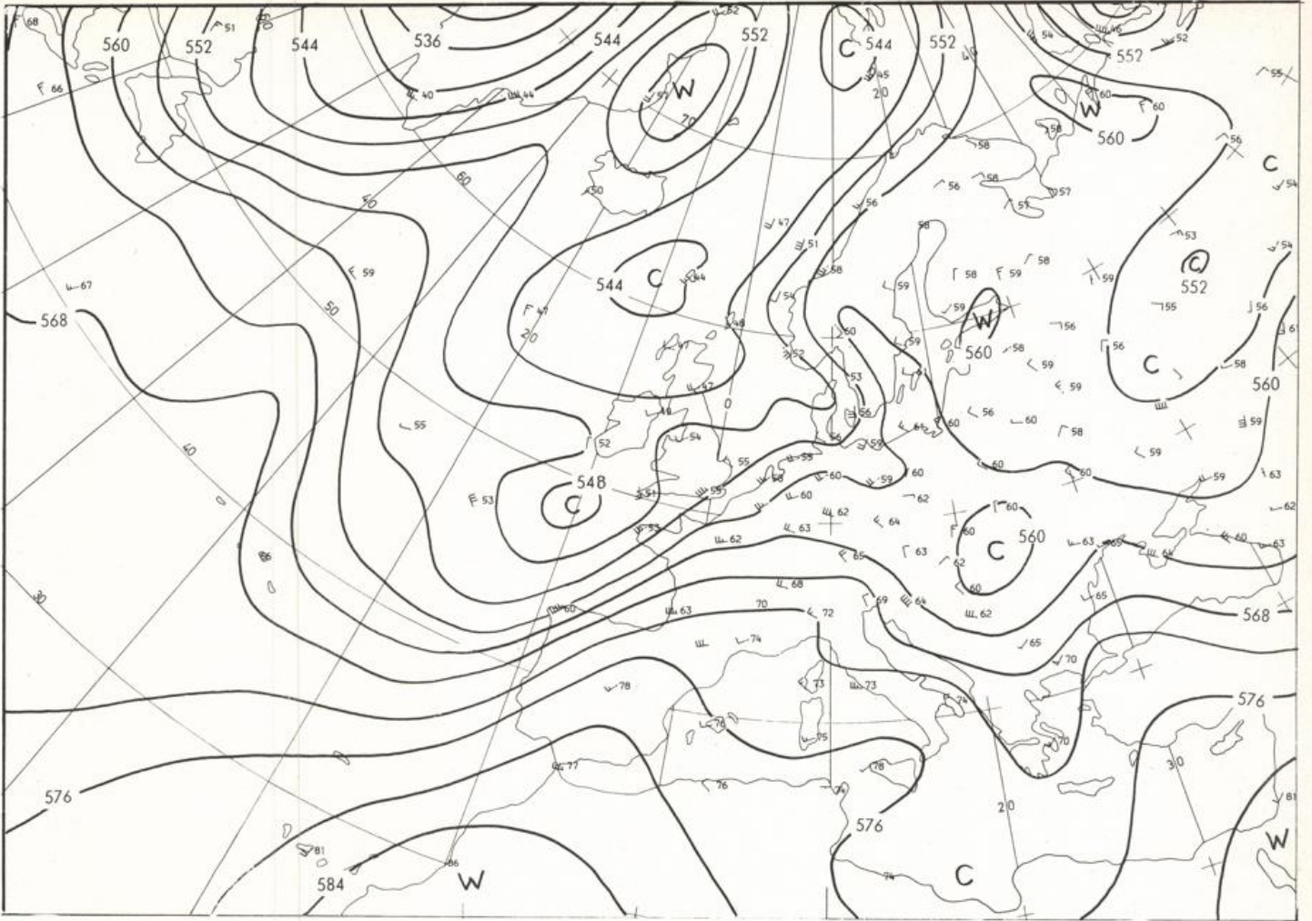
500/1000 hPa 00 GMT
