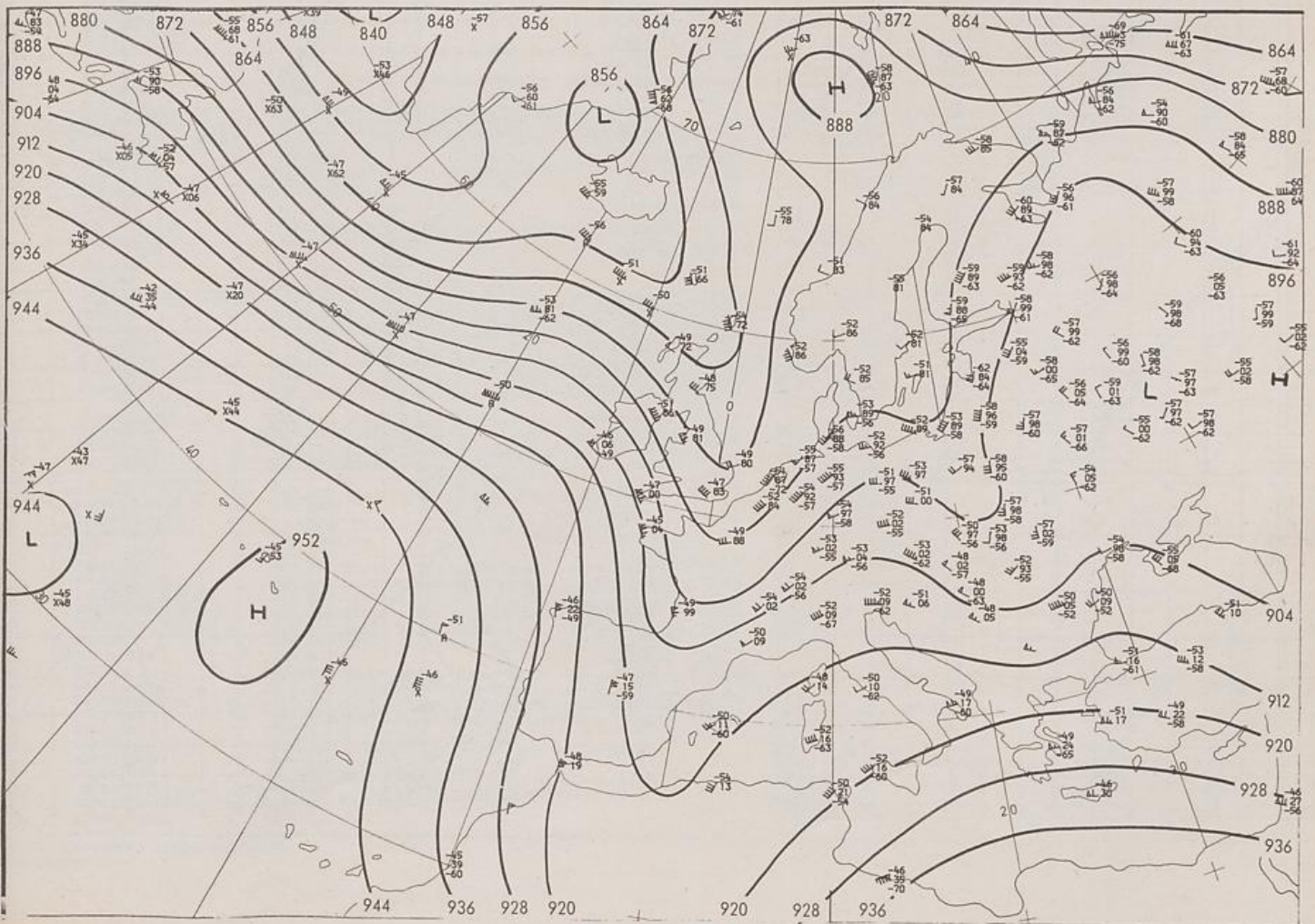
300 hPa 00 GMT
