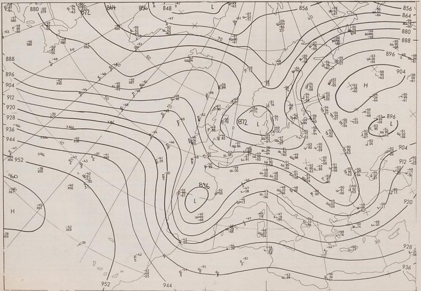
300 hPa 00 GMT
