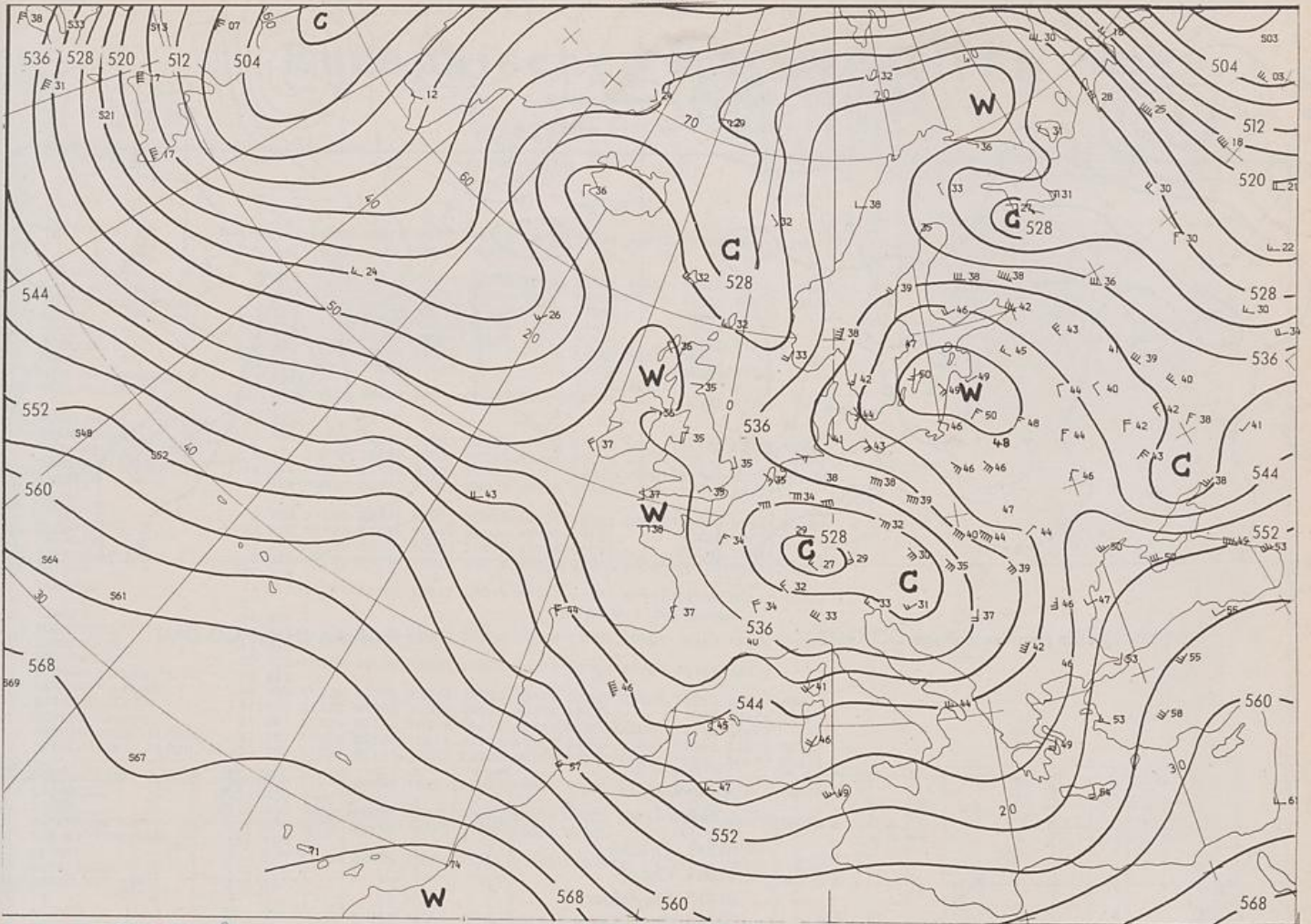
500/1000 hPa 00 GMT
