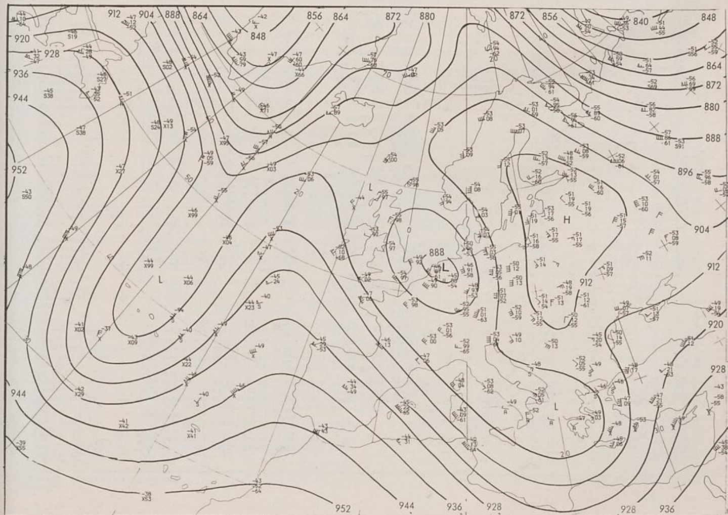
300 hPa 00 GMT
