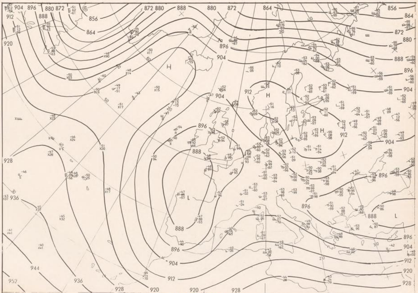
300 hPa 00 GMT
