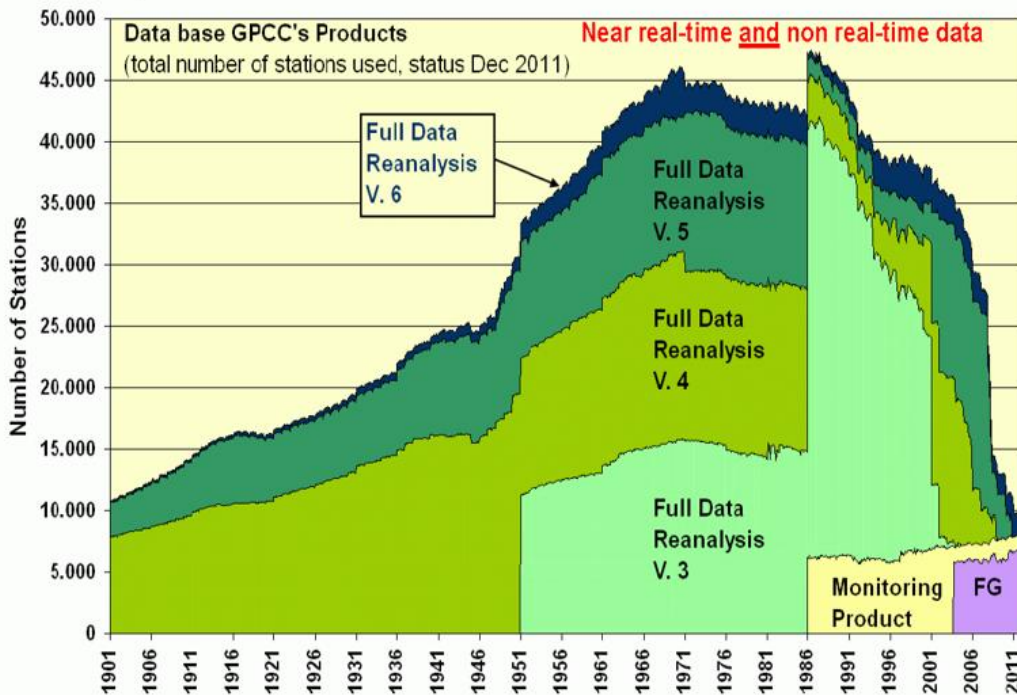
Figure 7: Total number of stations used for the GPCC products (Near real-time First-Guess Product, Monitoring Product, non real-time Full Data Reanalysis Product (Versions 3 to 6))
