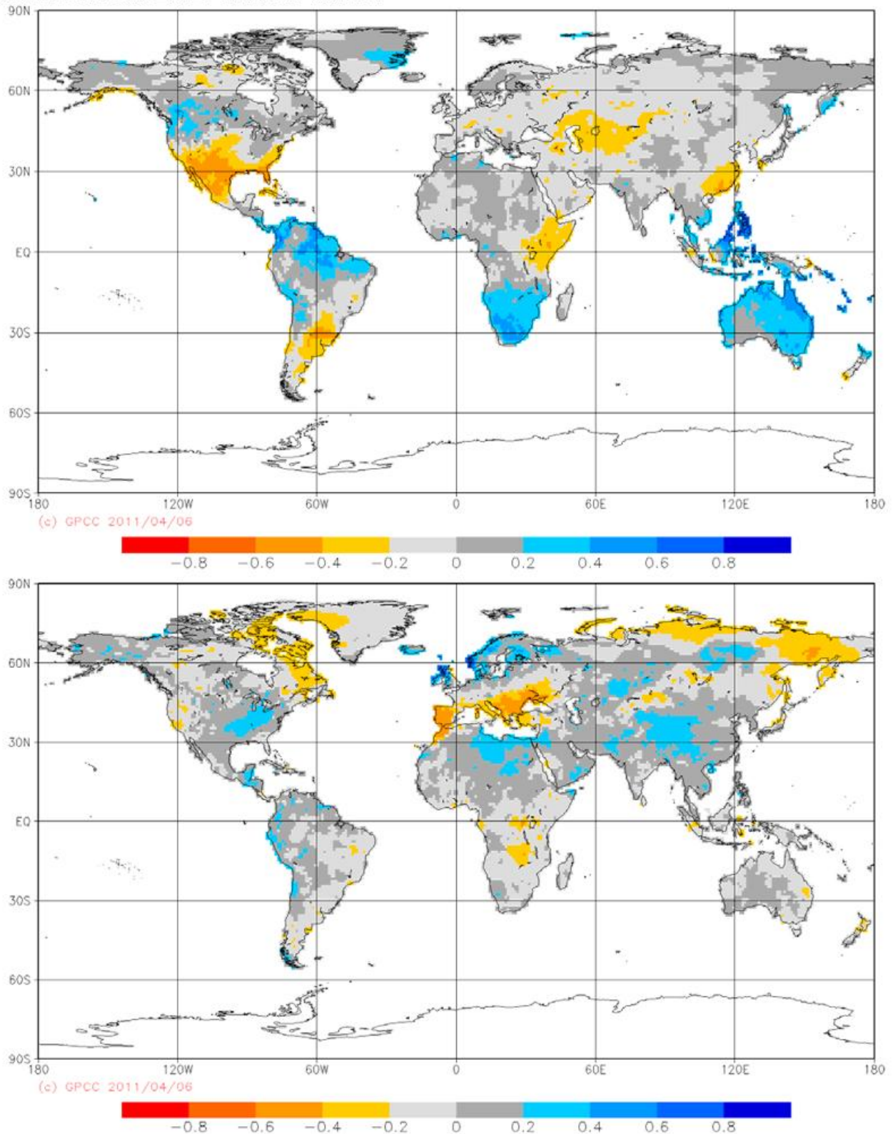
Figure 5: Correlation between monthly time series of gridded precipitation anomalies for the period 1901-March 2011 and (top) SOI and (bottom) NAO index (based on GPCC Full Data Reanalysis V.5, 0.5^\circ \times 0.5^\circ resolution, since Jan. 2010 Monitoring Product V.3)
