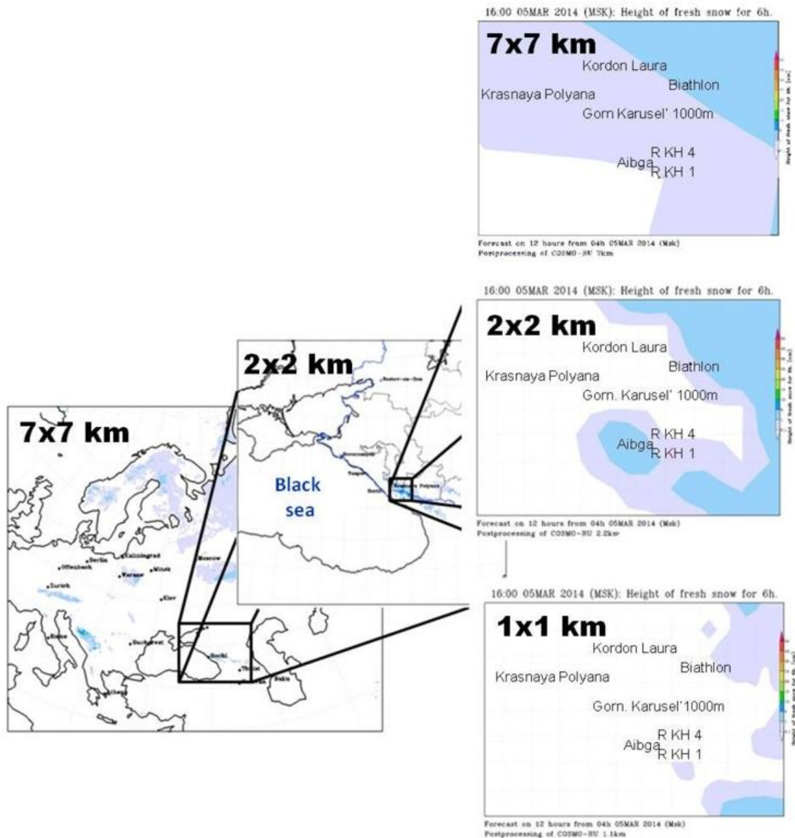
Figure 17: 12h-forecasts of fresh snow fallen for the last 6 hours according to COSMO-Ru7, COSMO-Ru2 and COSMO-Ru1. Start — 00 UTC 5 March 2014)
