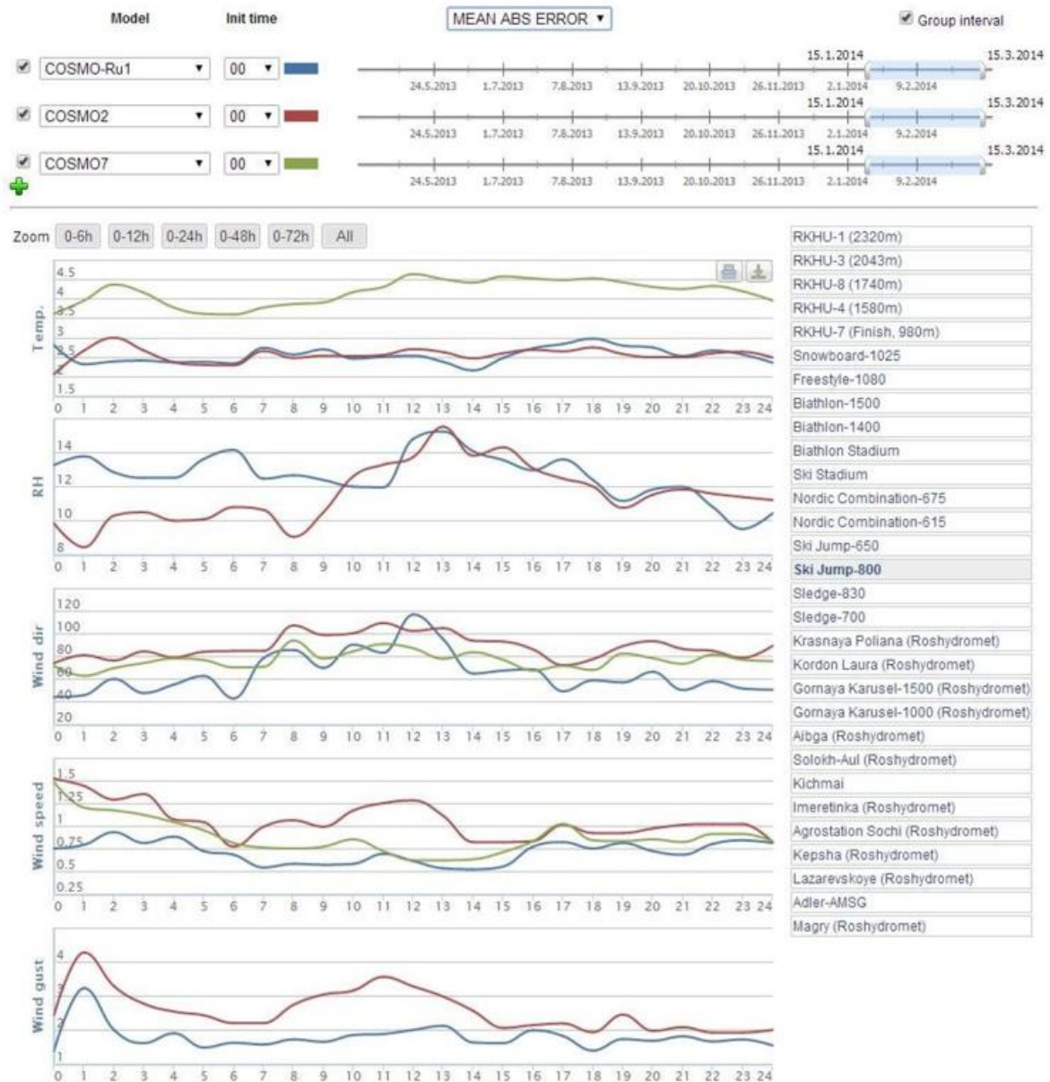
Figure 20: Effect of resolution, COSMO-Ru1, COSMO-Ru2, and COSMO-Ru7, 15 Jan–15 Mar 2014. Ski Jump-800 station
