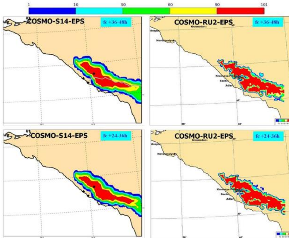
Figure 34: Probability of 12-hour snowfall exceeding 15 mm of equivalent water: COSMO-S14- EPS runs starting at 12 UTC of 11 January (top-left panel, t+36-48h) and at 00 UTC of 12 January (bottom-left panel, t+24-36h) and COSMO-Ru2-EPS runs starting at 12 UTC of 11 January (top-right panel, t+36-48h) and at 00 UTC of 12 January (bottom-right panel, t+24-36h). All forecasts verify at 12 UTC of 13 January 2013. As in Fig.33, the black squares in the left panels denote Sochi, Adler and Krasnaya Polyana.
