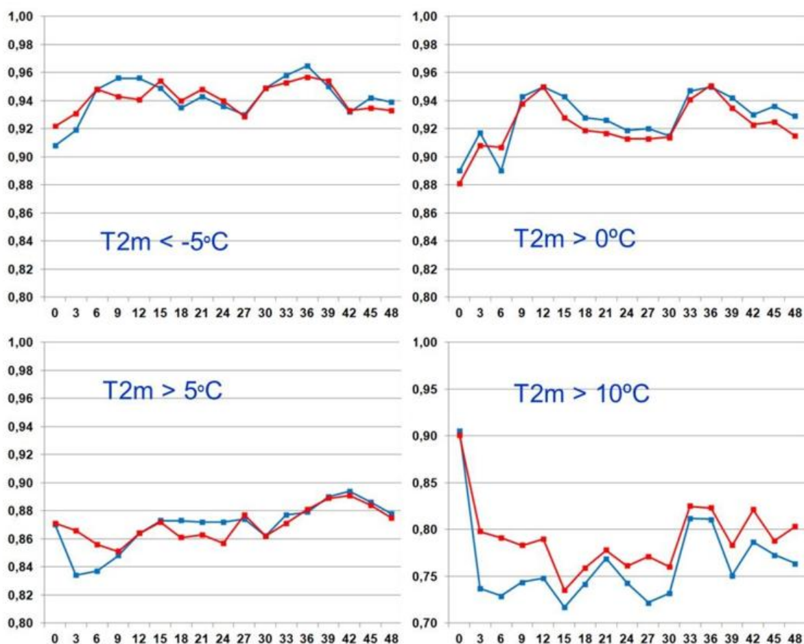
Figure 38: ROC area values as a function of forecast range for four different weather events: 2-metre temperature below -5^{\circ}\text{C} (top-left panel), above 0^{\circ}\text{C} (top right), above +5^{\circ}\text{C} (bottom left) and above +10^{\circ}\text{C} (bottom-right with different vertical scales). The scores are calculated over the period January-February 2013. Red (blue) lines refer to COSMO-S14-EPS (COSMO-Ru2-EPS)
