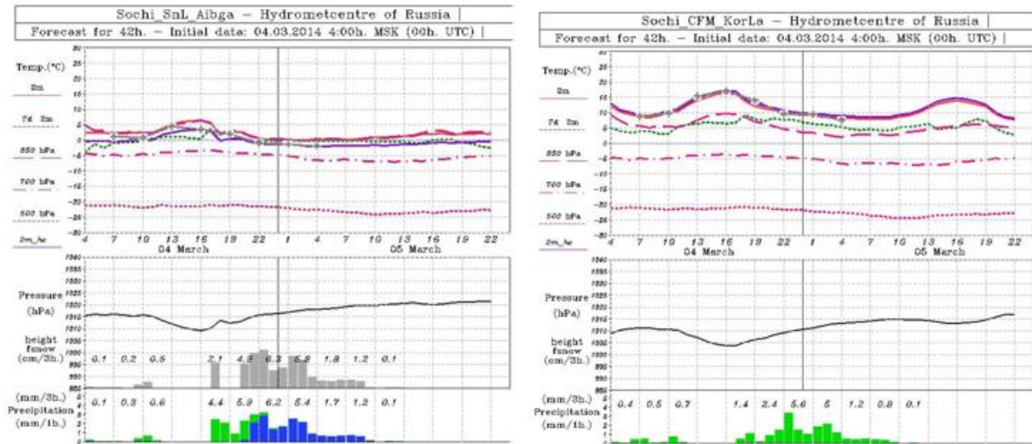
Figure 11: Example of meteograms obtained from integration of COSMO-Ru2 for station Aibga (left) and Kordon Laura (right). Start 00 UTC 4 March 2014. Height corrected temperature is presented by a violet curve, 2m temperature — pink line, result of KF application — gray dots. Grey columns show hourly accumulated depth of fresh snow, numbers above — its 3-hour sums. Blue columns indicate hourly accumulated precipitation in the form of snow, green — in the form of rain
