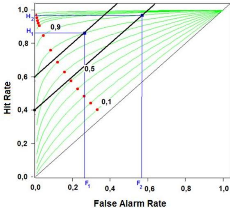
Figure 24: EDI (green) and PSS (black) isopleths; EDI for 0.1 – 0.9 and 0.95 – 0.99 with intervals 0.1 and 0.01; PSS = H - F for 0.4 and 0.6 values; H = F diagonal corresponds to EDI = PSS = 0. ; Red points: EDI curves tangent to straight PSS lines (strict formulas). Blue squares at (F,H): the monotonic EDI and PSS relation breaks down: Nonlinear dependence — not STRICTLY monotonic: for (F_1, H_1) and (F_2, H_2) PSS_1 > PSS_2 , but EDI_1 < EDI_2
