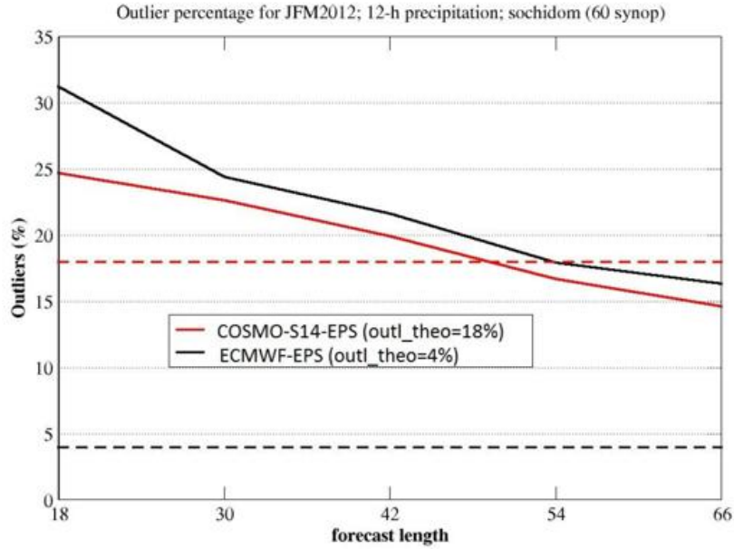
Figure 32: Percentage of Outliers for COSMO-S14-EPS (red) and ECMWF EPS (black), calculated over the 3-month period from January to March 2012. The red (black) dashed line indicates the theoretical limit of outliers for COSMO-S14-EPS (ECMWF EPS)
