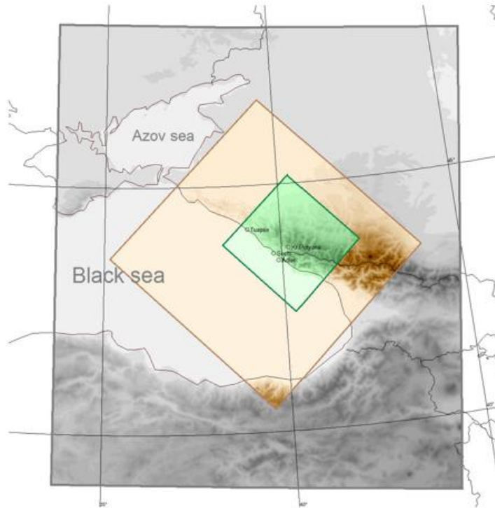
Figure 2: Location and size of COSMO-Ru2 domain (outer grey rectangle) and COSMO-Ru1 domains used in experiments: 450 x 450 grid points (brown-colored square) and 200 x 200 grid points (inner green-colored square)
