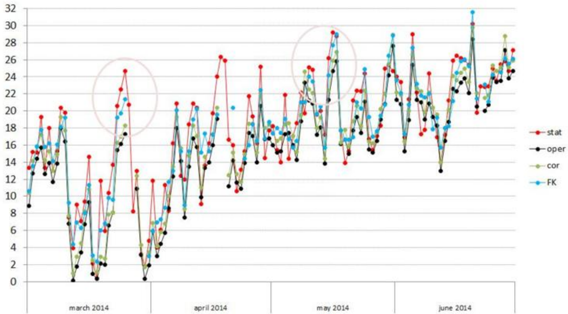
Figure 14: Example of T2m 12h forecasts by COSMO-Ru2 for station Krasnaya Polyana. Start 00 UTC. 1 March — 30 June 2014. Red line observations, black — operational forecast, green — T2m correction algorithm, blue — Kalman filtering
