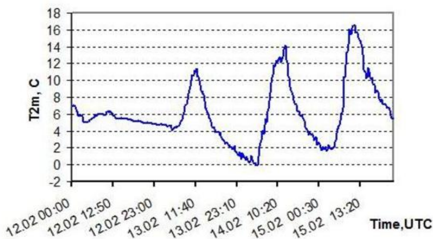
Figure 35: Behavior of 2-metre temperature in Krasnaya Polyana (10-min data of the automatic meteorological station)
