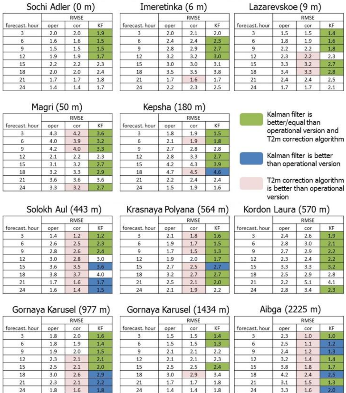
Figure 13: RMSE for T2m COSMO-Ru2 forecasts for stations in the Sochi region. Start 18 UTC. 1 March — 30 June 2014
