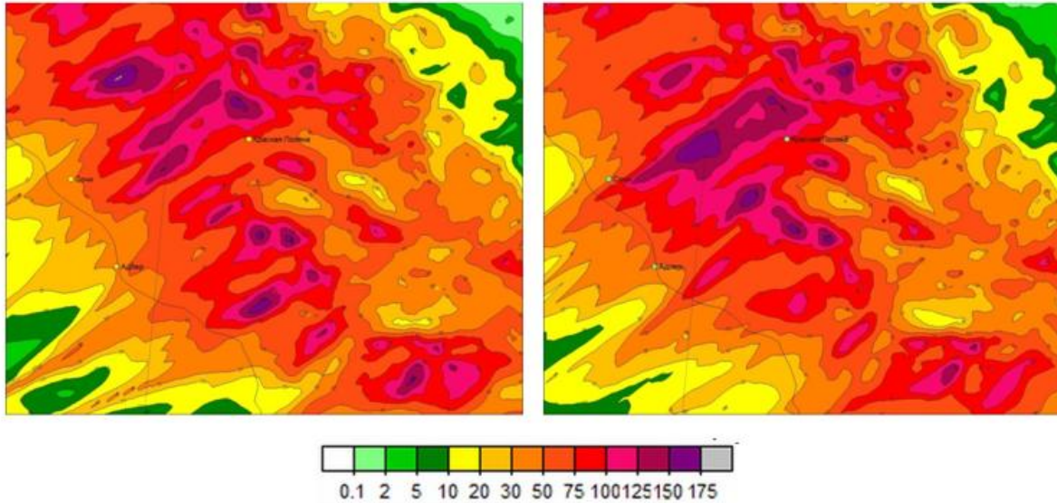
Figure 4: The same as figure 3 but for 12h precipitation sum
