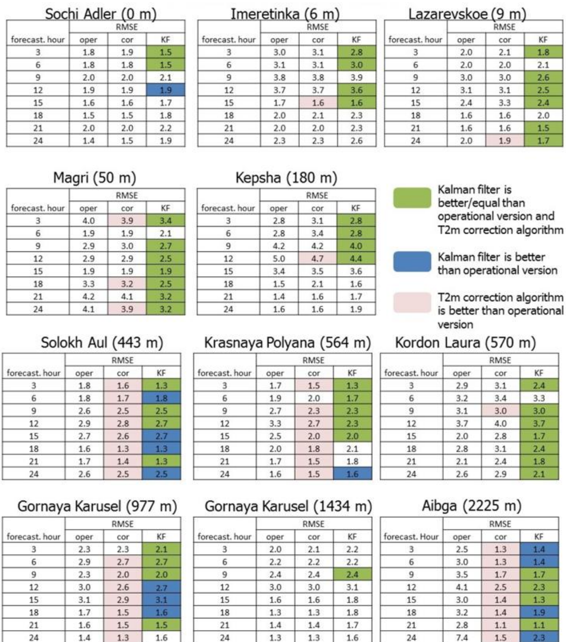
Figure 12: RMSE for T2m COSMO-Ru2 forecasts for stations in the Sochi region. Start 00 UTC. 1 March — 30 June 2014
