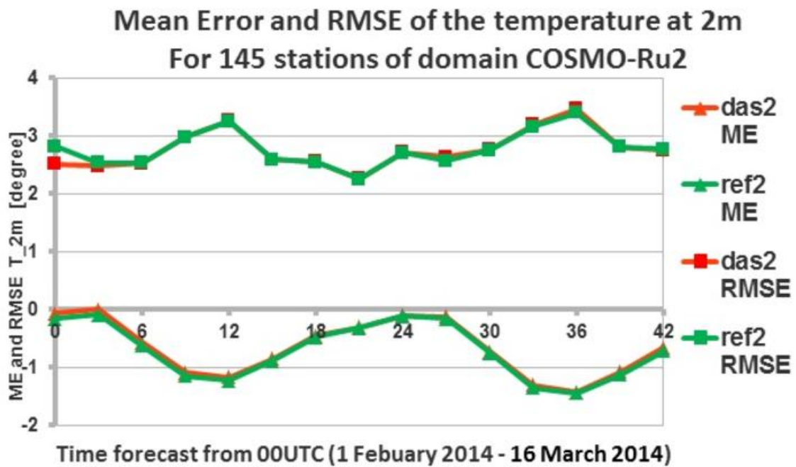
Figure 1: Mean error (ME) and Root Mean Square Errors (RMSE) of forecasts COSMO-Ru2 with DAS (red line) and without (green line) for PMSL, T_{2m} , Td_{2m} and wind speed respectively for Olympic period 1 February – 16 March 2014
