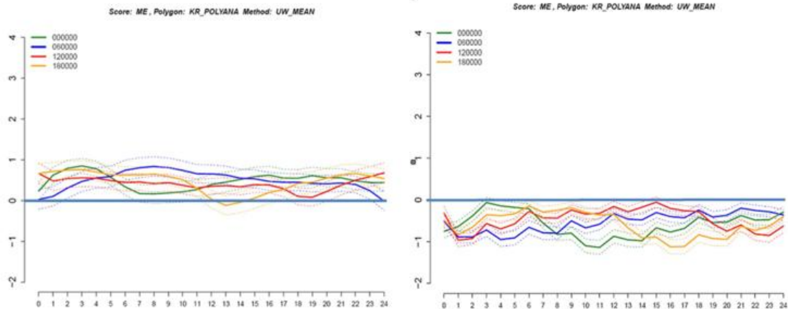
Figure 21: COSMO2Ru T2m mean error during the first test period (winter 2012–2013) (left panel) and the second test period (Jan–Feb 2014) (right panel) (all initial times) at Krasnaya Polyana station
