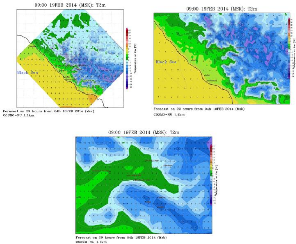
Figure 7: COSMO-Ru1 output presentation example. T2m forecast for the entire simulation domain (upper left), the Sochi region (upper right) and mountain cluster (bottom)
