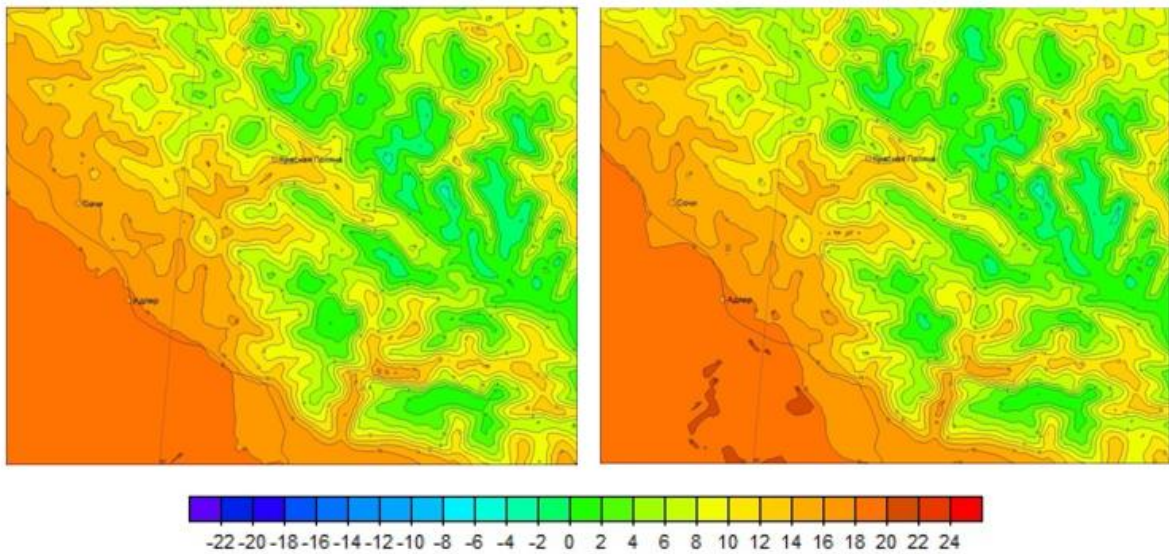
Figure 3: T2m 12 h forecasts from 24.09.2013, 00 UTC obtained in experiments with simulations domain 200 x 200 grid points (left) and 450 x 450 grid points (right)
