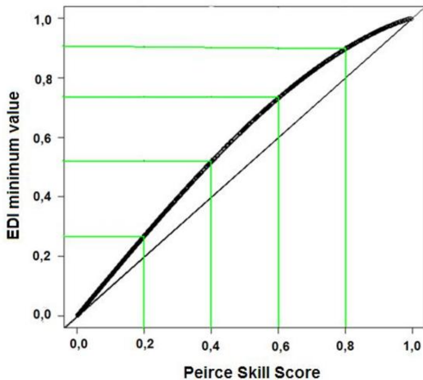
Figure 25: Relation between EDI minimum value and PSS
