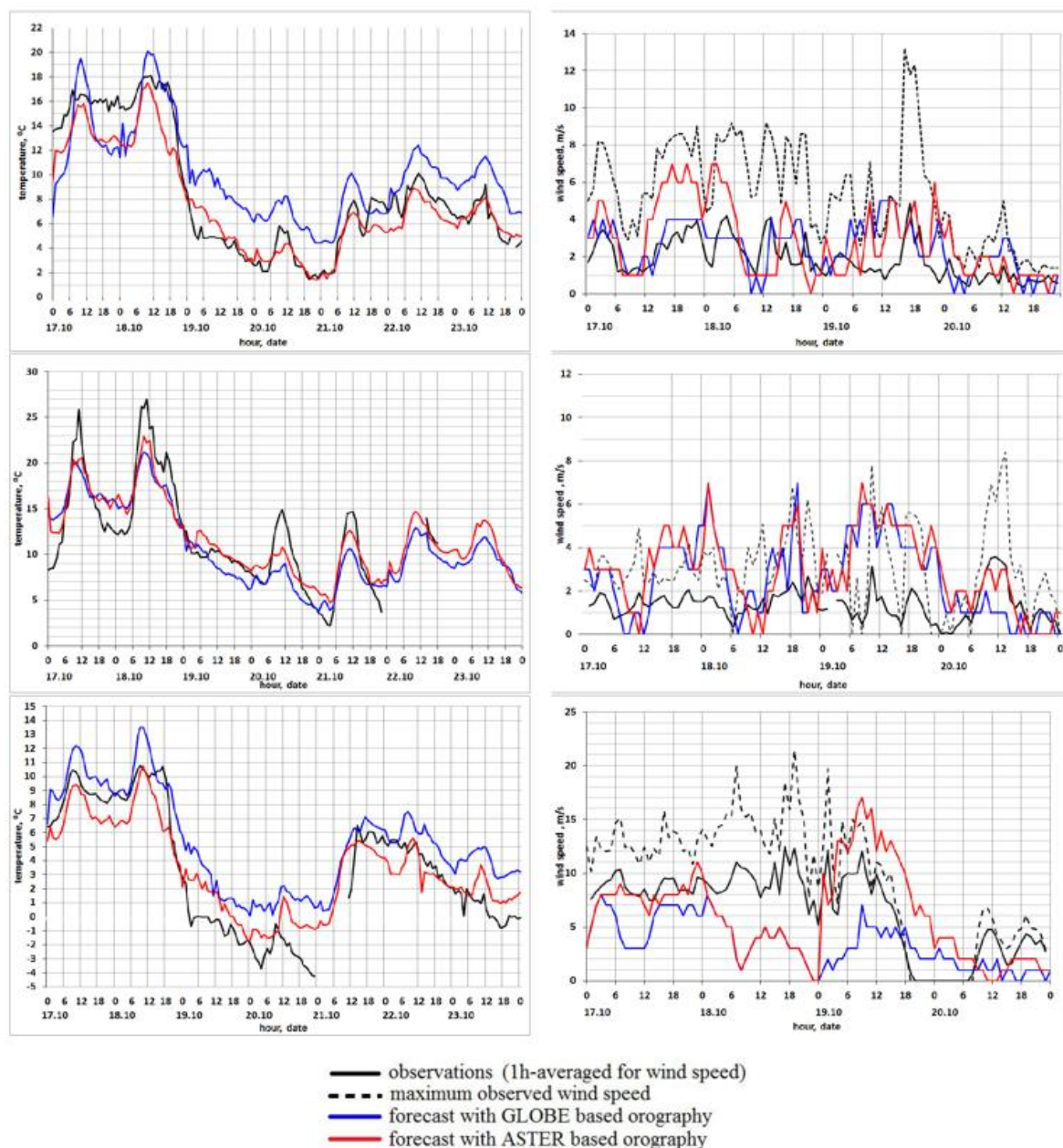
Figure 5: Series of 24 h forecasts for T2m (left) and wind speed at 10 m (right) from 00 UTC, for the period October, 17-23, 2013 (for T2m) and October, 17-20 (for wind) and observation data at Gornaya Karusel (top), Krasnaya Polyana (middle) and Aibga (bottom) for the same period
