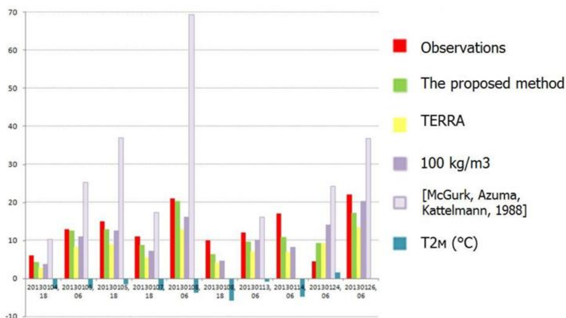
Figure 15: Fresh snow depth (cm) is coloured as: red observations at station Gornaya Karusel, light green results of proposed method using T2m ( ^{\circ}\text{C} ), yellow using formula from TERRA of the COSMO-model, violet under the assumption of the constant fresh snow density value of 100 \text{ kg/m}^3 , light violet according to linear dependency on T700. In blue T2m values ( ^{\circ}\text{C} ) are shown
