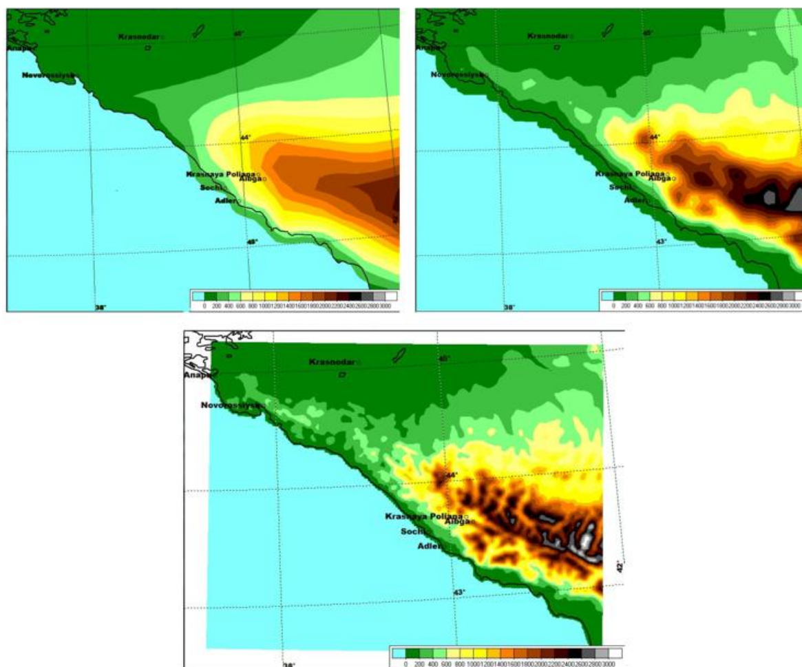
Figure 27: Model orography (in m) for ECMWF-EPS ( \Delta x = 31 km, top-left panel), COSMO-S14-EPS ( \Delta x = 7 km, top-right panel) and COSMO-RU2-EPS ( \Delta x = 2.2 km, bottom panel) in the Olympic region
