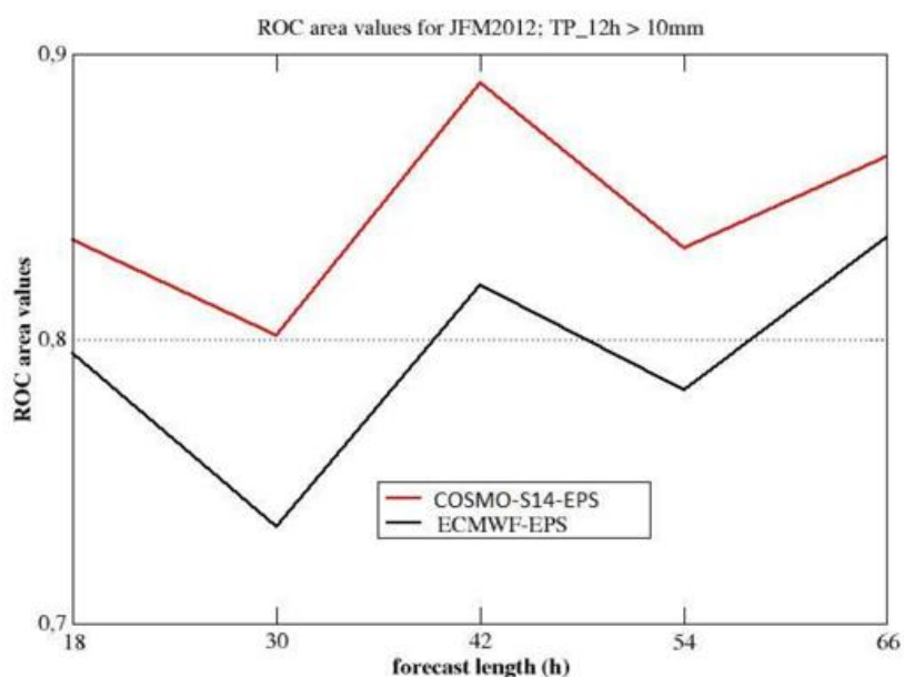
Figure 31: ROC area values for COSMO-S14-EPS (red) and ECMWF EPS (black) relative to the event “precipitation exceeding 10mm in 12 hours” for the forecast ranges of Table 8. Both scores are calculated over the 3-month period from January to March 2012
