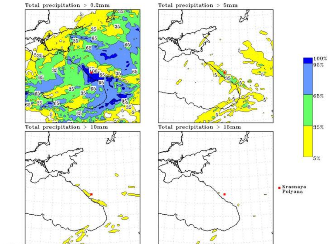
Figure 28: An example of COSMO-S14-EPS products operationally provided to the Olympic forecasters: probabilities of the events “3-h cumulated precipitation is more than 0.2 (upper left panel), 5 (upper right panel), 10 (lower left panel), and 15 mm (lower right panel)”. COSMO-S14-EPS 45-h forecast starting from 10 March 2014, 00 UTC. A red square indicates the location of Krasnaya Polyana
