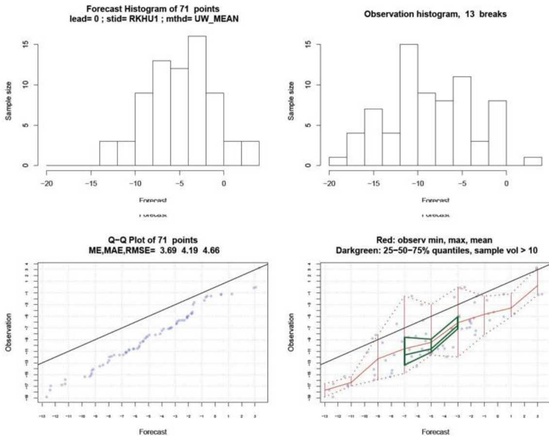
Figure 22: An example of diagnostic verification plots
