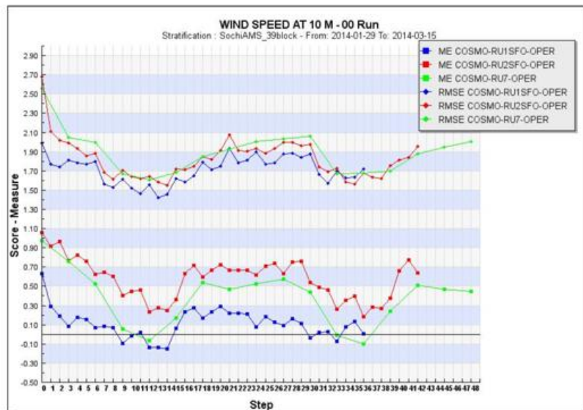
Figure 8: Verification COSMO-Ru1 (blue), COSMO-Ru2 (red) and COSMO-Ru7 (green) results for the 39 stations located at different altitudes in the mountain and coastal clusters for the period 29.01.2014 15.03.2014
