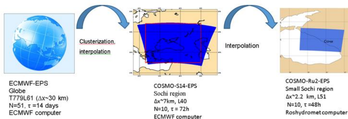
Figure 26: Organization of COSMO ensemble forecasting for the Sochi region. N is the ensemble size, \tau is the forecast length, and L is the number of vertical levels
