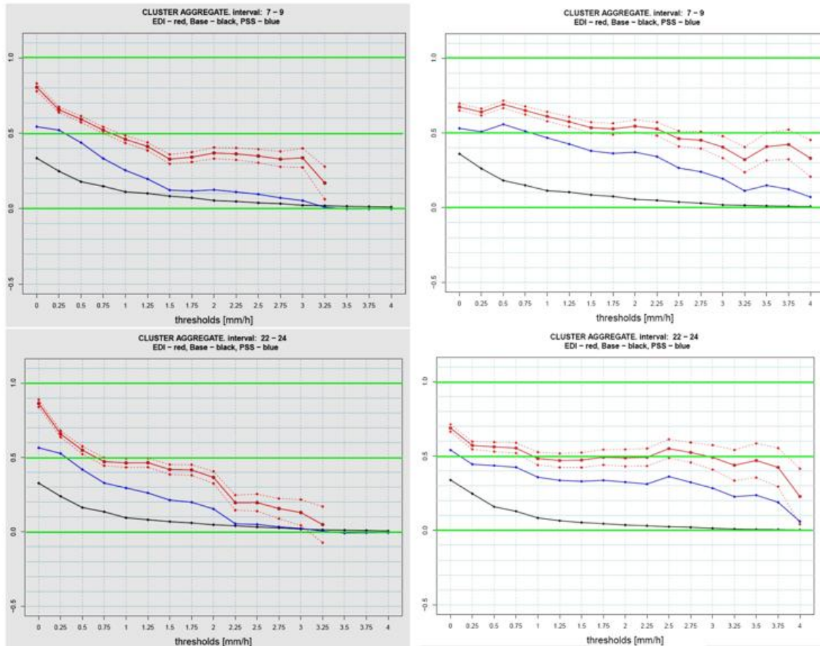
Figure 23: EDI (red), PSS (blue), and base rate (black) for COSMO-Ru2 (left panel, shaded) and NMMB (right panel) 3h precipitation, nearest point, Jan–March 2013, Mountain cluster
