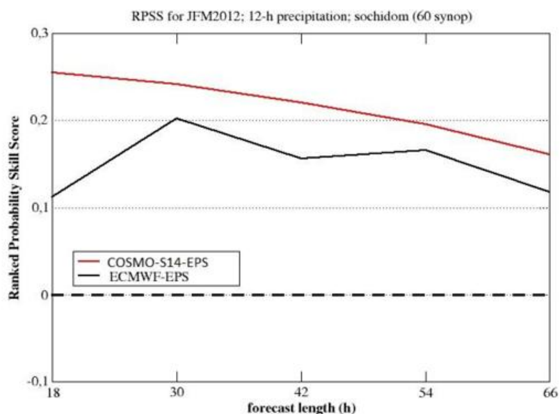
Figure 30: Ranked Probability Skill Score as a function of forecast length for COSMO-S14-EPS
