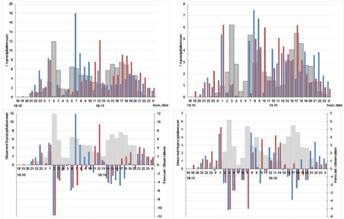
Figure 6: 1 h observed accumulated precipitation (grey column), forecasted by COSMO-Ru1 with different model orography: based on GLOBE data (blue) and ASTER data (red) for Gornaya Karusel-1500 (left) and Krasnaya Polyana (right). Comparison of 1h accumulated precipitation (top) and difference of two forecasts (bottom)
