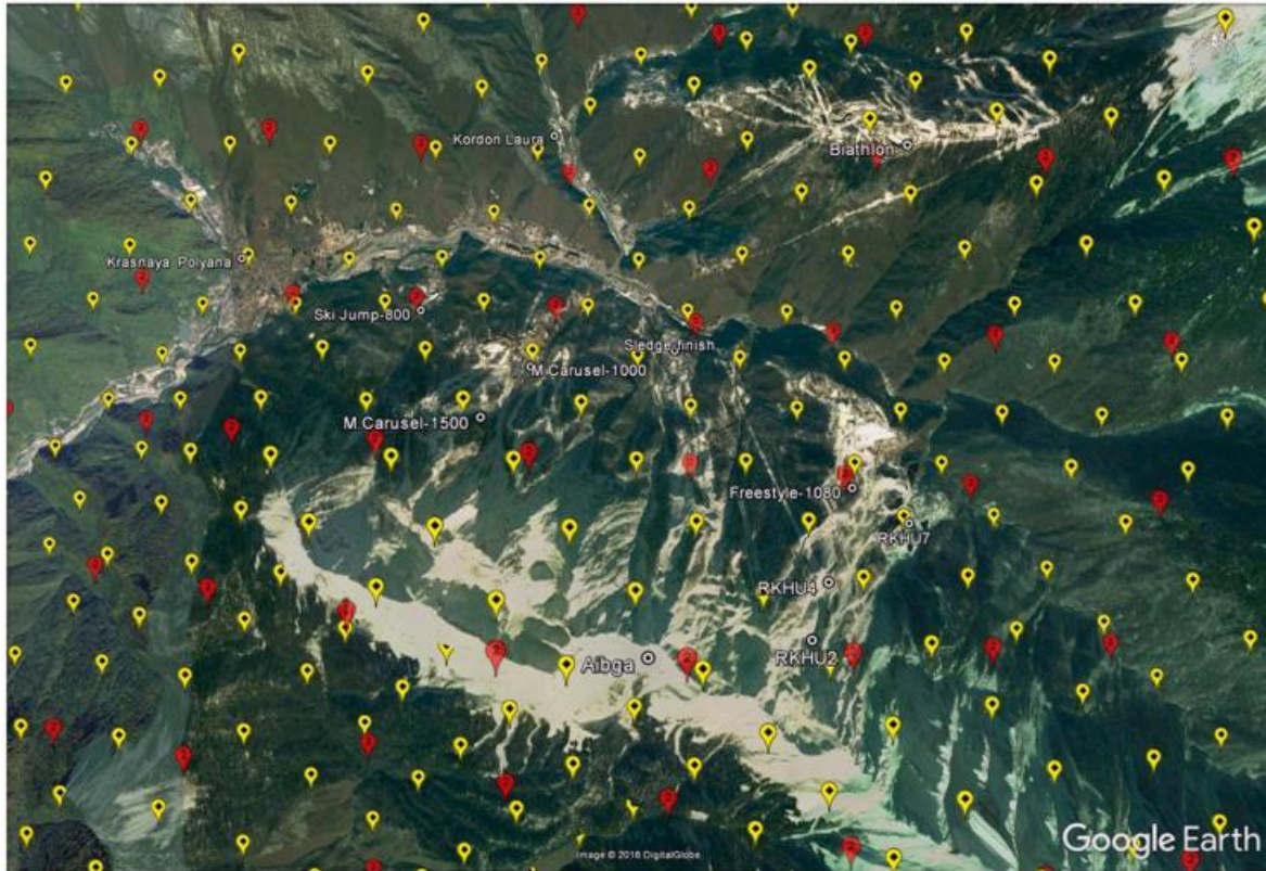
Figure 18: Nearest point approach: COSMO-RU2 (red lamps) and COSMO-Ru1 (yellow points) — models grid points and weather stations (superscripted)
