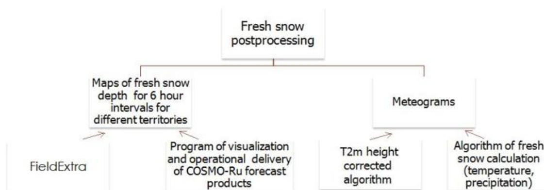
Figure 16: The scheme of fresh snow depth calculation at Hydrometcenter of Russia (based on mesoscale model COSMO-Ru)
