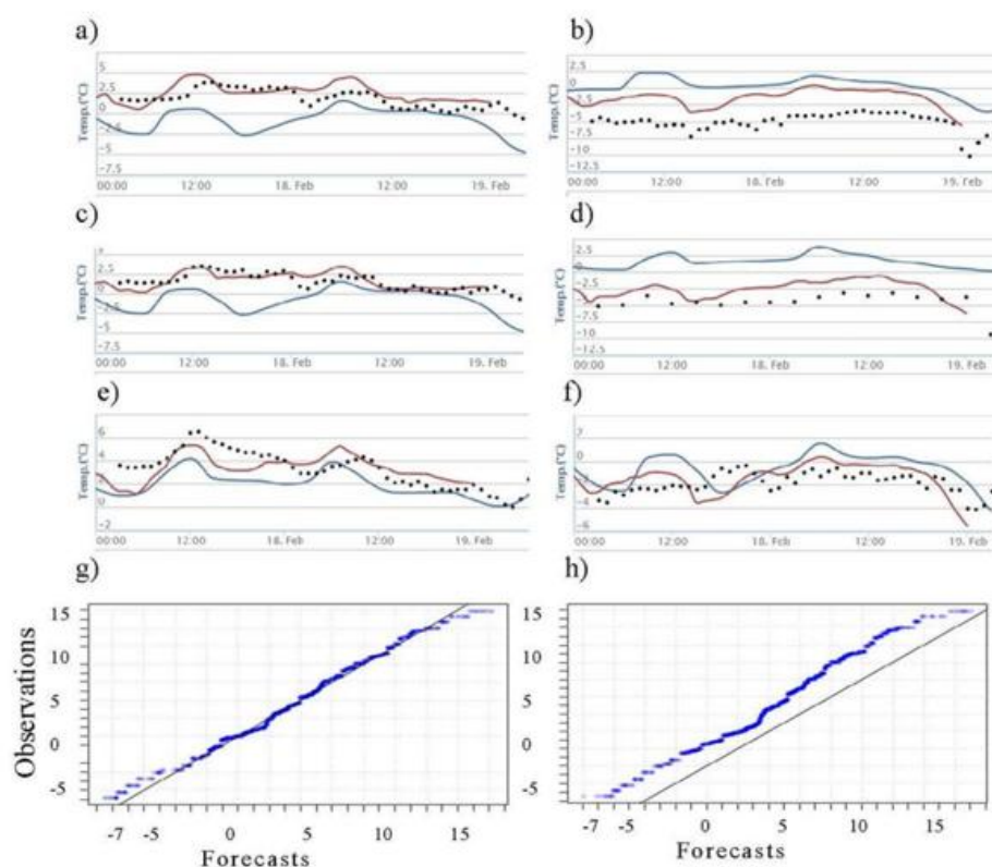
Figure 40: Ensemble mean 2-m temperature predicted by COSMO-Ru2-EPS (in red) and COSMO-S14-EPS (in blue) and observed (black dotted line) at mountain stations RKHU-7 (980 m) (a), RKHU-1 (2320 m) (b), Snowboard-1025 (1027 m) (c), Aibga (2225 m) (d), Sledge-700 (701 m) (e), Gornaya Karusel-1500 (1434 m) (f) using the analysis on 18 February 2014, 00 UTC; quantile-quantile plots for 24-h forecasts of COSMO-Ru2-EPS (g) and COSMO-S14-EPS (h) and observations at RKHU-7 station for the period from January 15 to March 15, 2014
