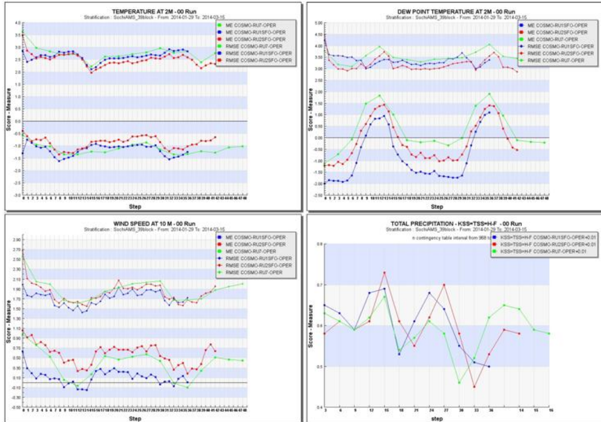
Figure 19: Scores for COSMO-Ru1, COSMO-Ru2, and COSMO-Ru7, 29 Jan–15 March 2014
