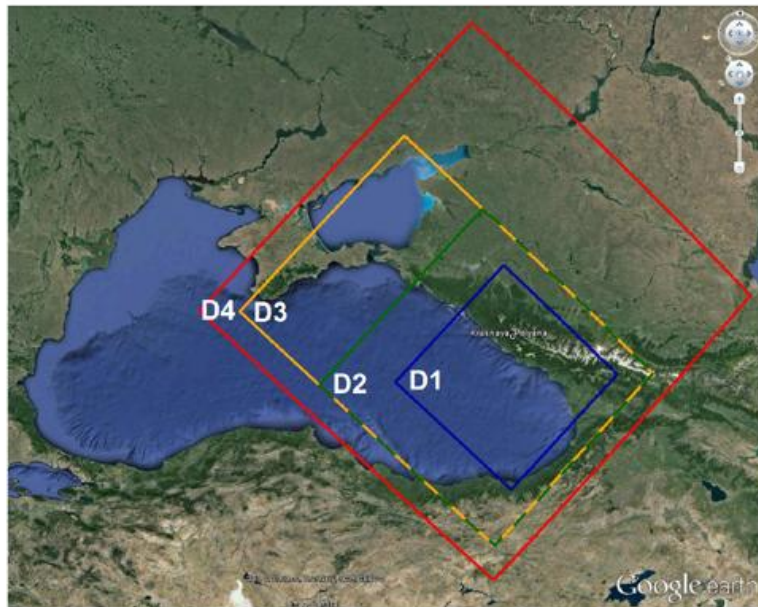
Figure 2: Simulation domains: D1 (blue rectangle) 300 \times 300 grid points, D2 (green rectangle) 450 \times 450 grid points, D3 (yellow rectangle) 450 \times 650 grid points, D4 (red rectangle) 750 \times 750 grid points.
