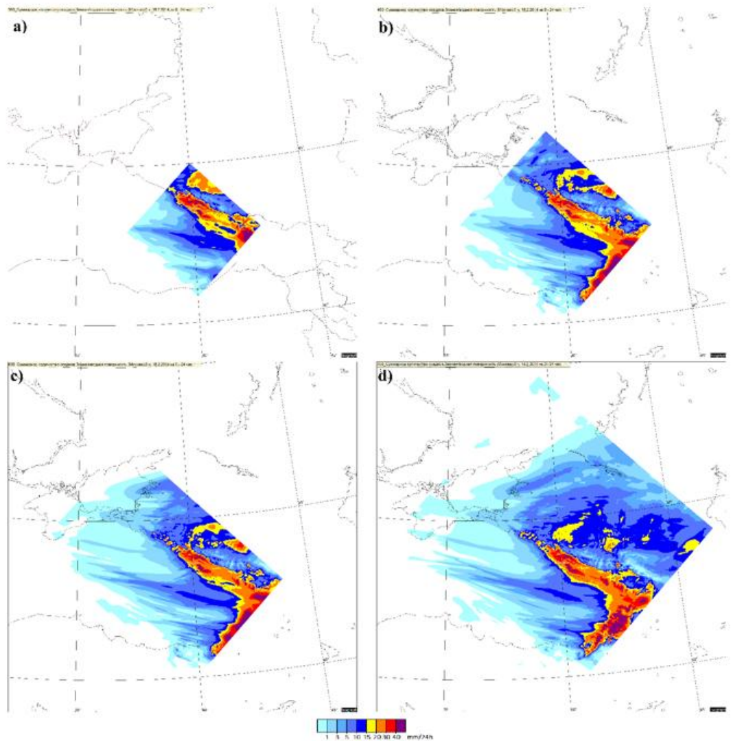
Figure 8: 24 hours accumulated precipitation predicted for various domains: D1 (a), D2 (b), D3 (c), D4 (d). Forecast start 18.02.2014, 00 UTC.
