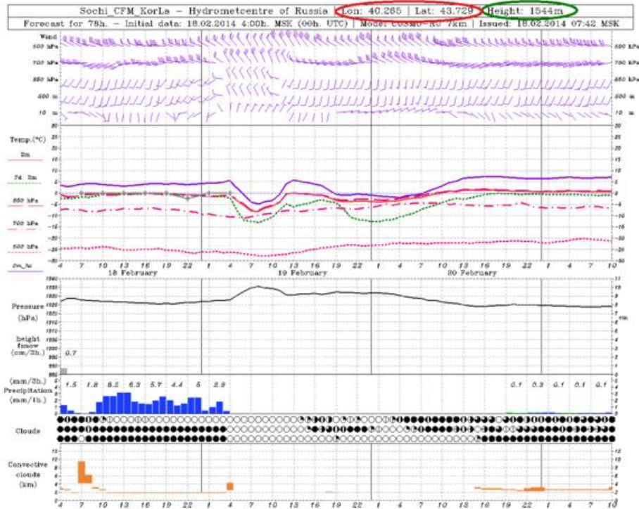
Figure 26: Example of meteogram for Cordon Laura. The coordinates and high of grid- box are circled in ovals (red and green).
