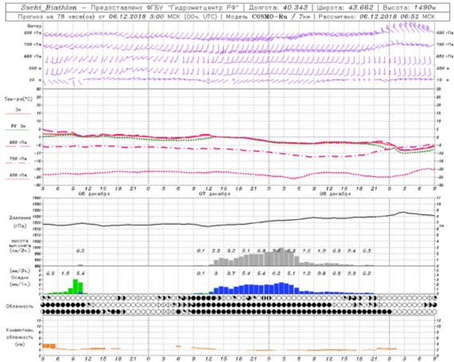
Figure 24: Example of deterministic meteogram for points of Sochi mountain.
